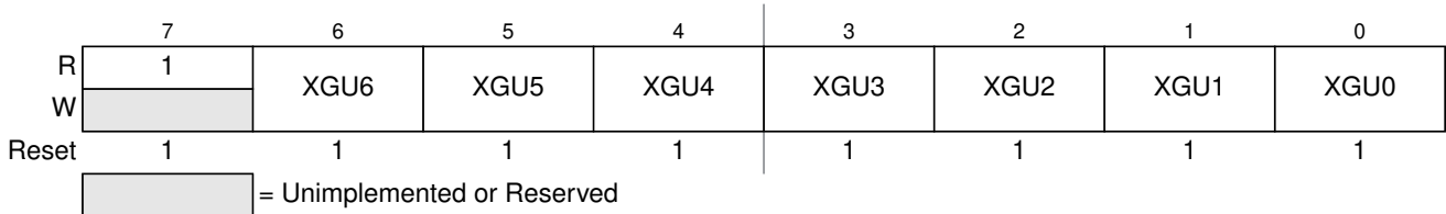
Figure 17-18. RAM XGATE Upper Boundary Register (RAMXGU)
