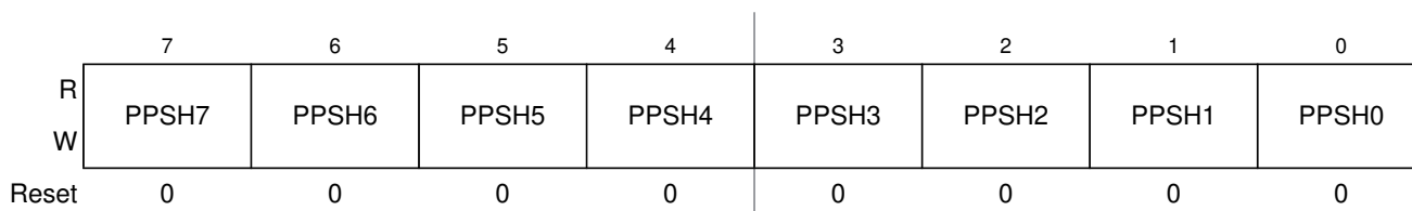
Figure 24-49. Port H Polarity Select Register (PPSH)
