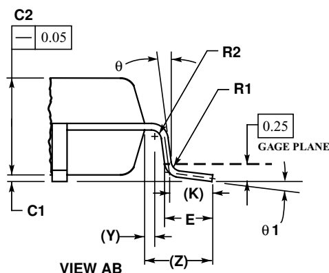
Figure B-1. 144-Pin LQFP Mechanical Dimensions (Case No. 918-03)
