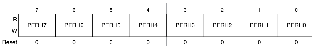
Figure 24-48. Port H Pull Device Enable Register (PERH)
