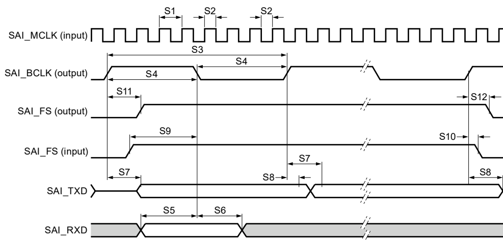
Figure 54. SAI controller mode
