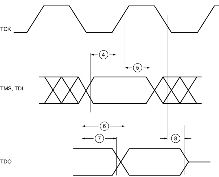
Figure 74. JTAG Test Access Port Timing
