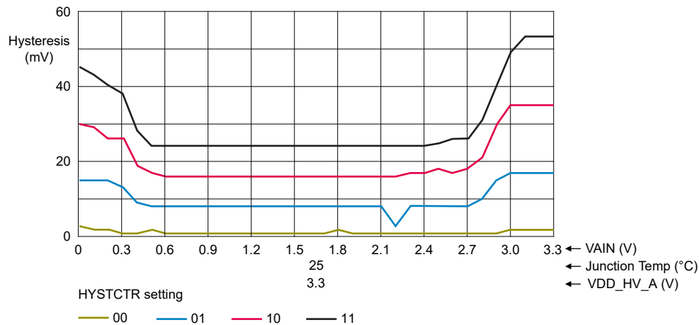
Figure 43. Typical Hysteresis vs VAIN (VDD_HV_A = 3.3 V, Low Speed Mode)
