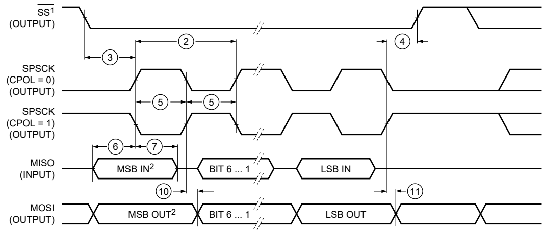
Figure 50. LPSPI Controller Mode Timing (CPHA=0)
