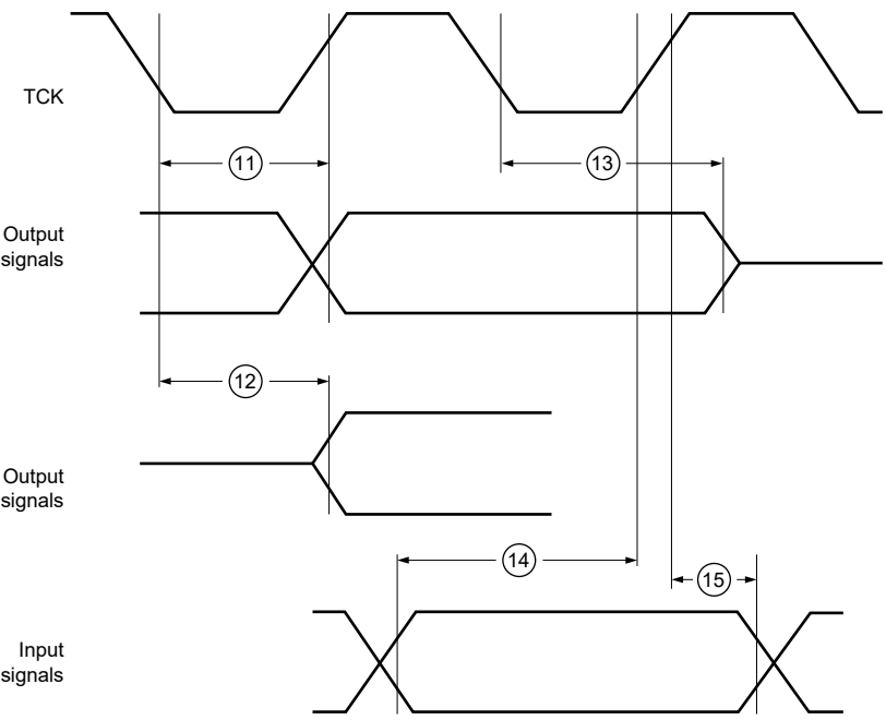
Figure 75. Boundary Scan Timing
