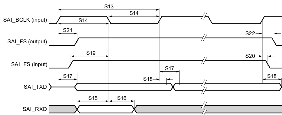
Figure 53. SAI target mode
