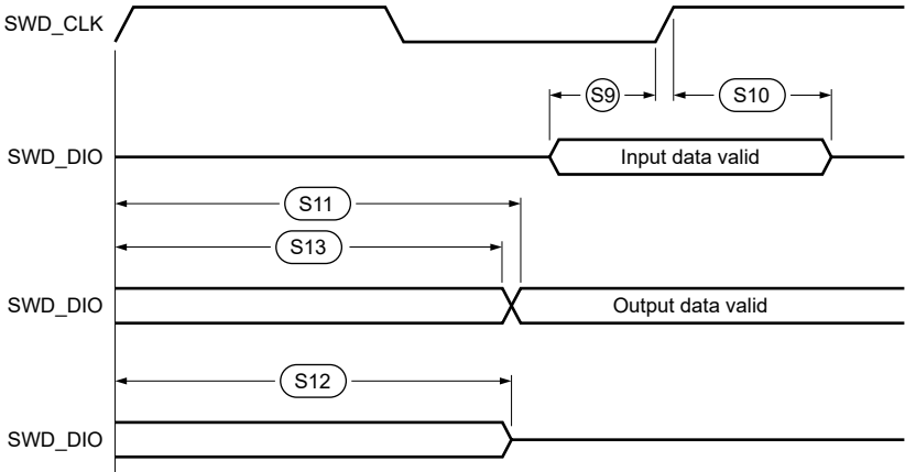
Figure 72. SWD Output Data Timing
