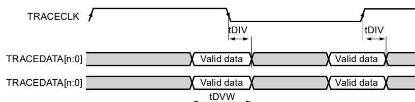
Figure 70. Trace CLKOUT specifications
