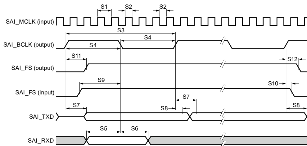
Figure 54. SAI controller mode
