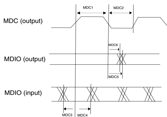
Figure 63. MII/RMII serial management channel timing
