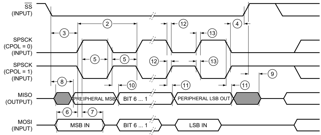
Figure 49. LPSPI Peripheral Mode Timing (CPHA=0)
