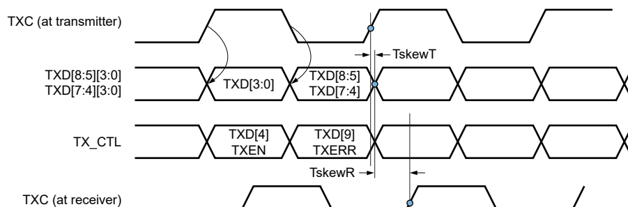
Figure 62. RGMII Transmit Timing
