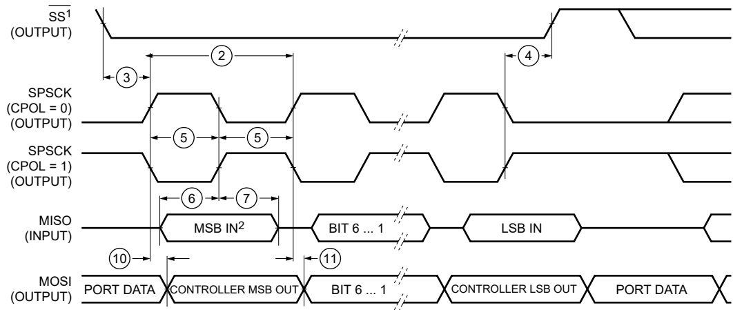
Figure 51. LPSPI Controller Mode Timing (CPHA=1)
