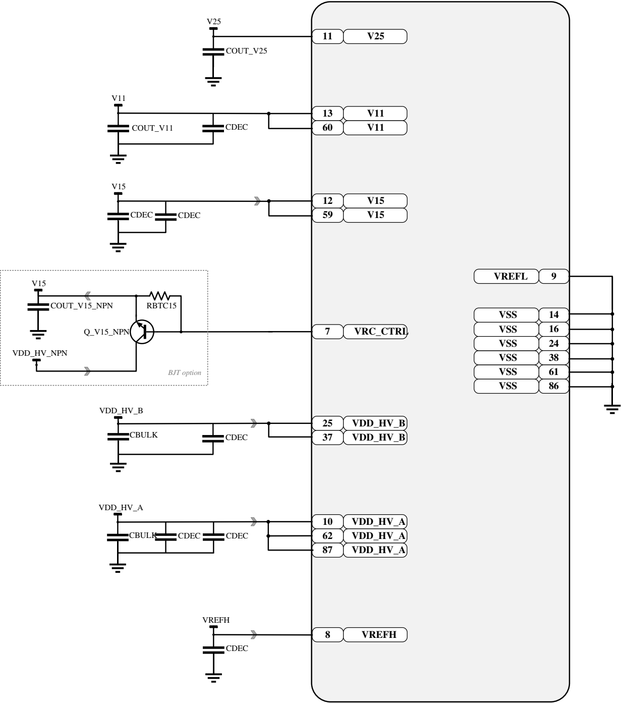
Figure 32. 100LQFP package decoupling capacitor pinout diagram, (S32K344, S32K324, S32K314)
