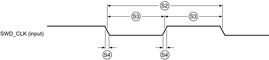
Figure 71. SWD Input Clock Timing
