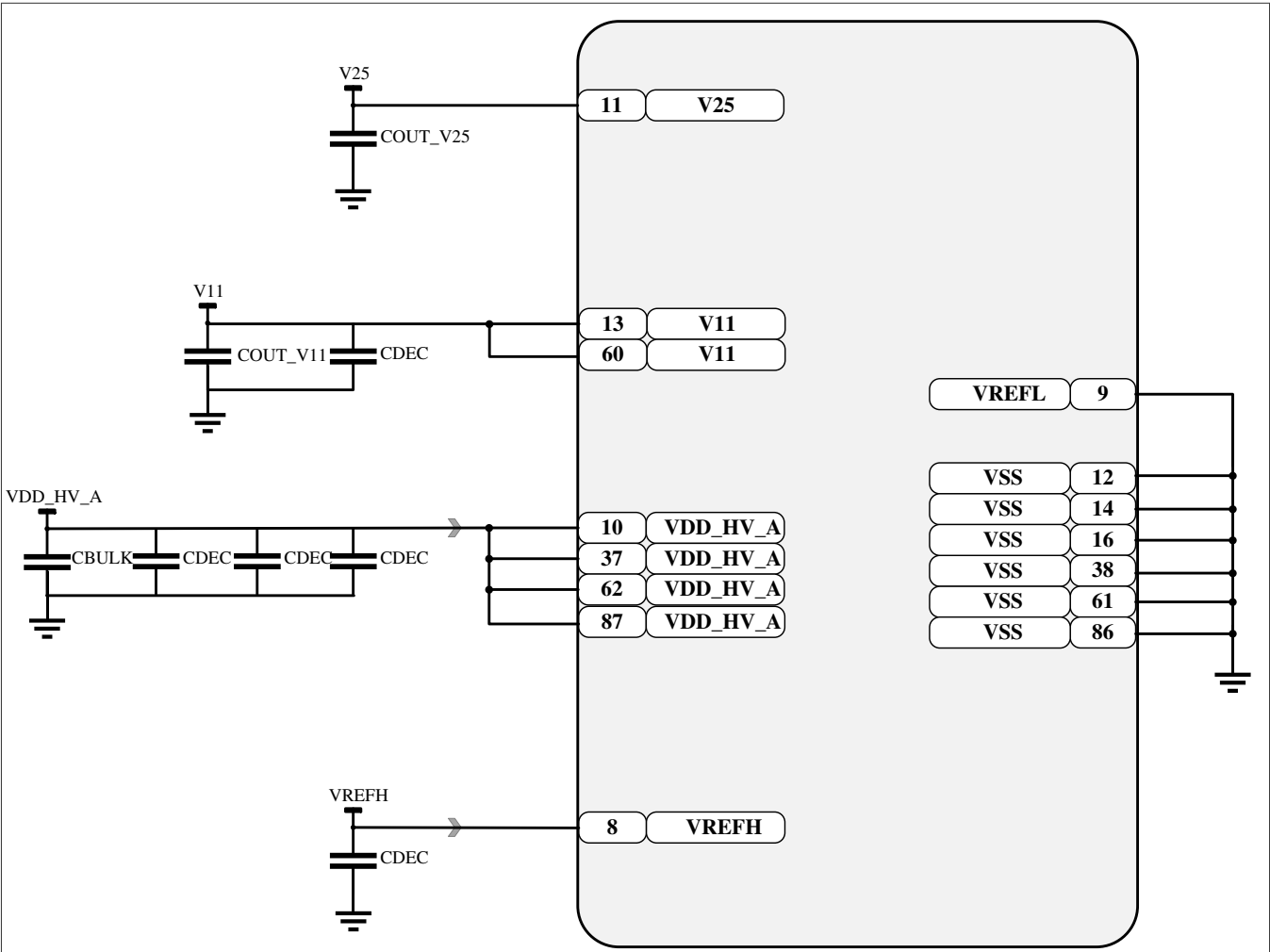
Figure 33. 100LQFP package decoupling capacitor pinout diagram, (S32K312)
