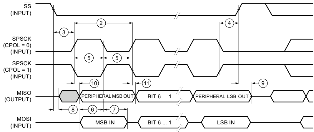
Figure 48. LPSPI Peripheral Mode Timing (CPHA=1)
