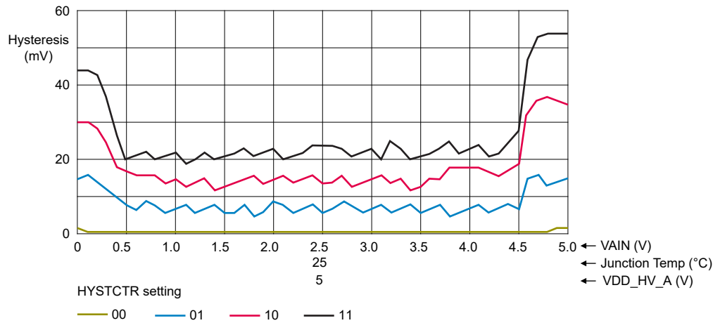
Figure 45. Typical Hysteresis vs VAIN (VDD_HV_A = 5 V, Low Speed Mode).png
