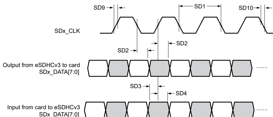
Figure 69. SD/eMMC4.4/4.41 DDR50 Mode Interface Timing
