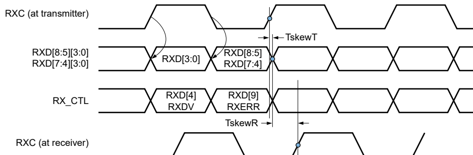
Figure 61. RGMII Receive Timing
