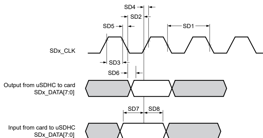
Figure 68. SD/eMMC4.3 High Speed Mode Interface Timing
