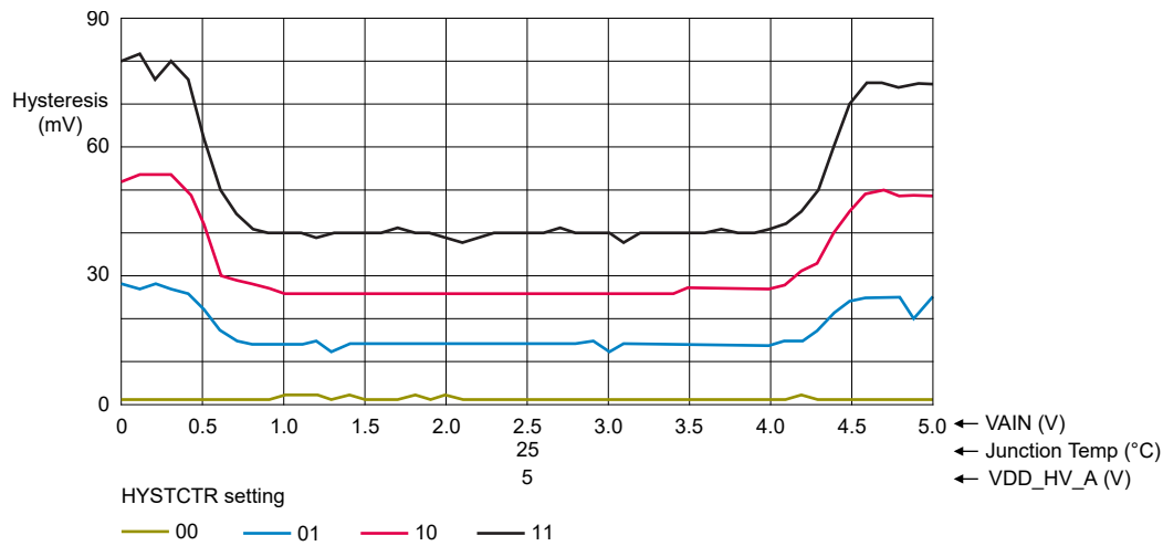
Figure 44. Typical Hysteresis vs VAIN (VDD_HV_A = 5 V, High Speed Mode).png
