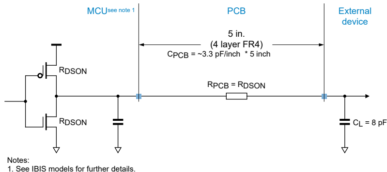
Figure 37. Reference Load Diagram
