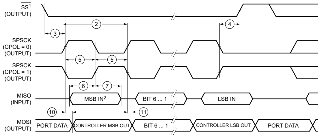
Figure 51. LPSPI Controller Mode Timing (CPHA=1)
