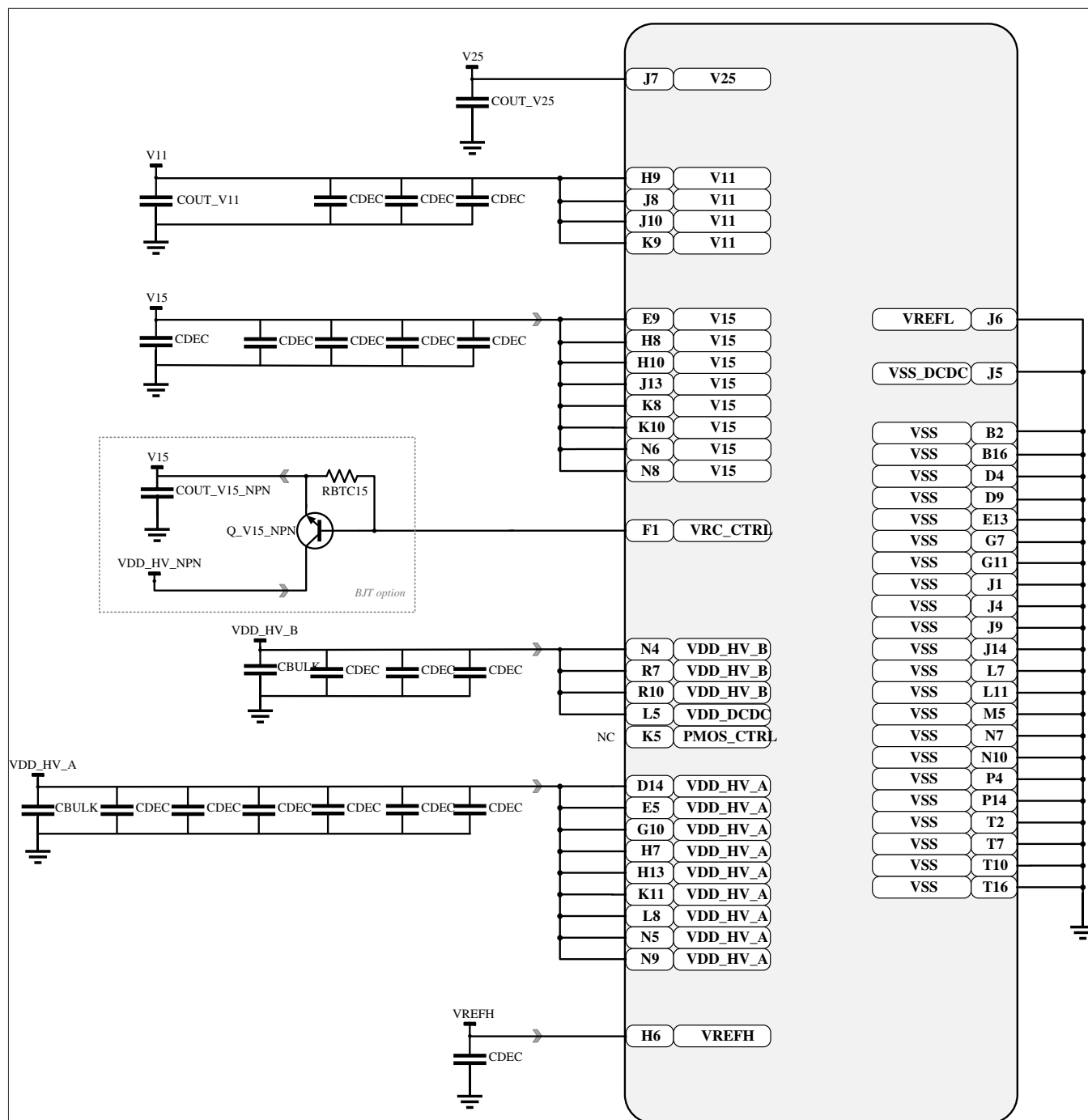
Figure 26. 289BGA package decoupling capacitor pinout diagram (S32K358, S32K356, S32K348, S32K338 and S32K328)
