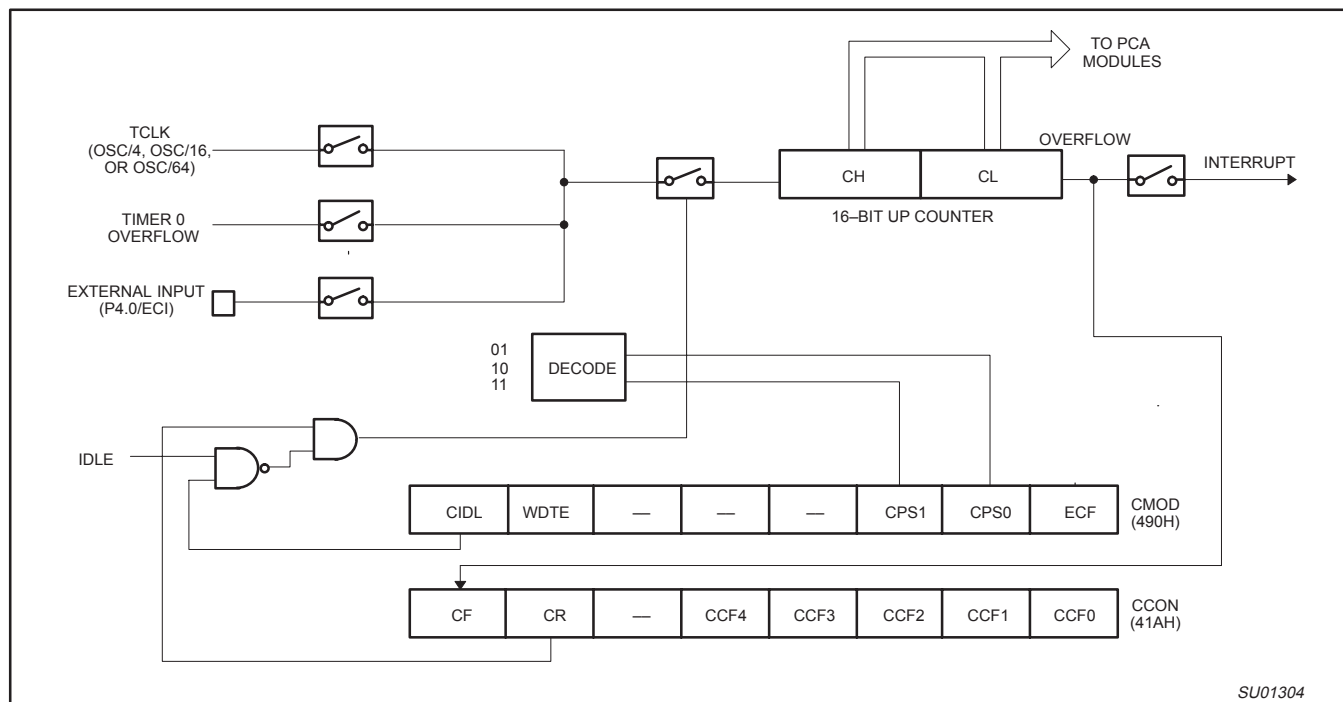
Figure 8. PCA Timer/Counter
