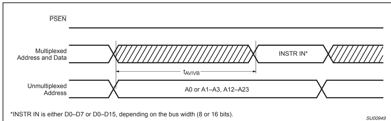
Figure 27. External Program Memory Read Cycle (Non-ALE Cycle)
