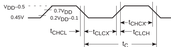
Figure 22. External Clock Drive
