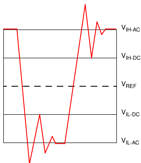
Figure 3: SSTL_2 Receiver Signal Conditions
