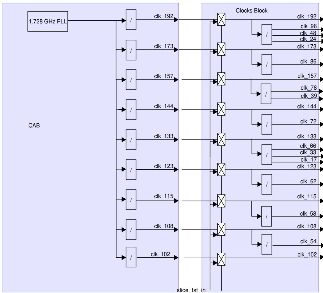
Figure 10: Clock Dividers
