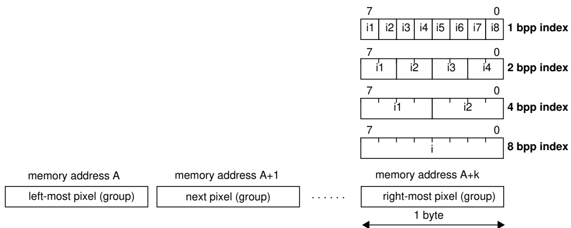
Figure 2: Indexed Formats
