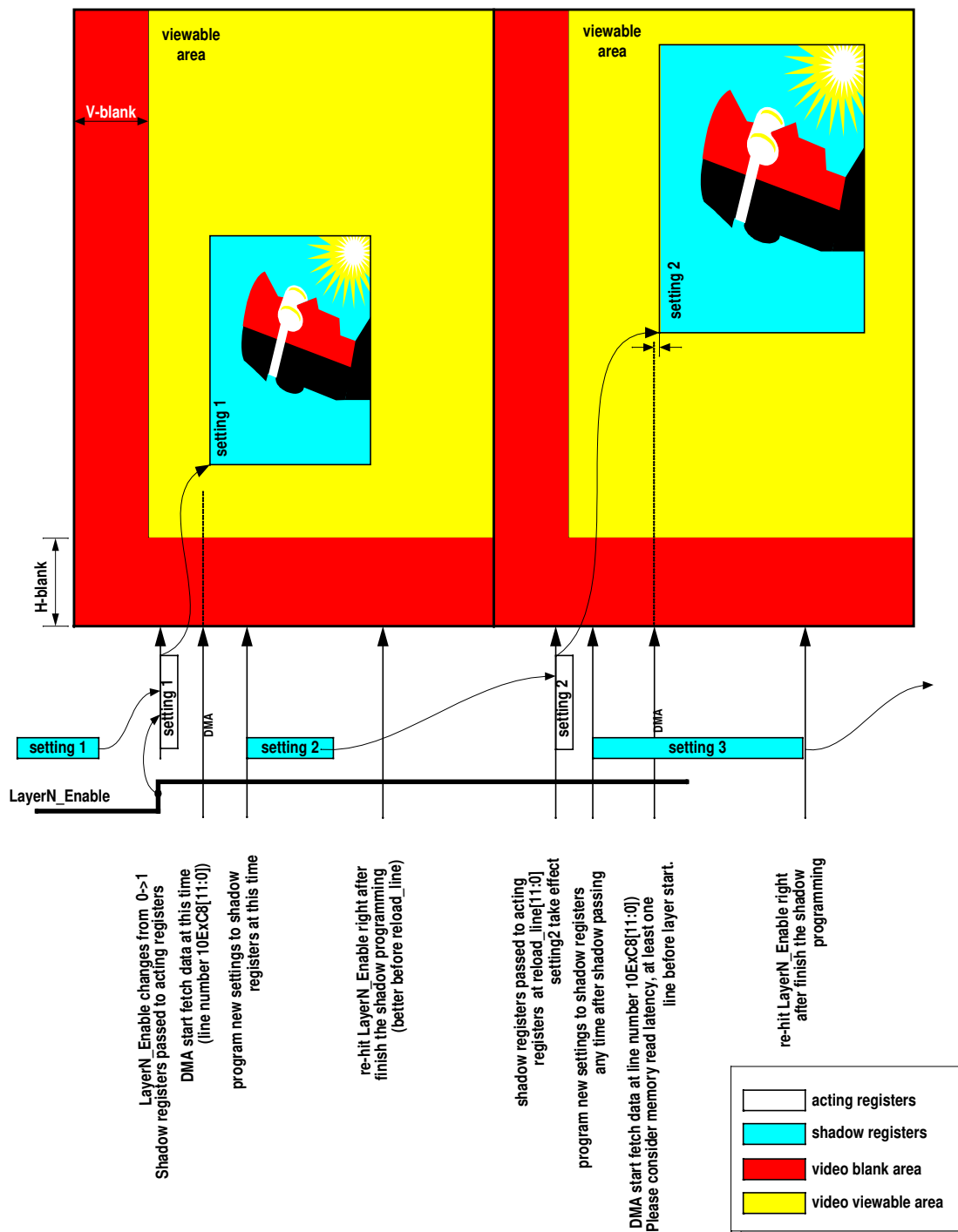
Figure 8: Shadow Mechanism
