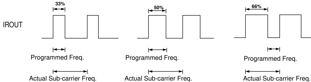
Figure 11: Examples of Duty Cycles for Ir TX Signals
