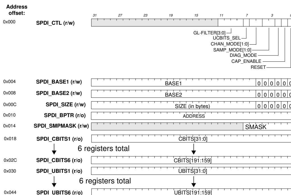
Figure 9: SPDIF Input MMIO Registers (1 of 2)
