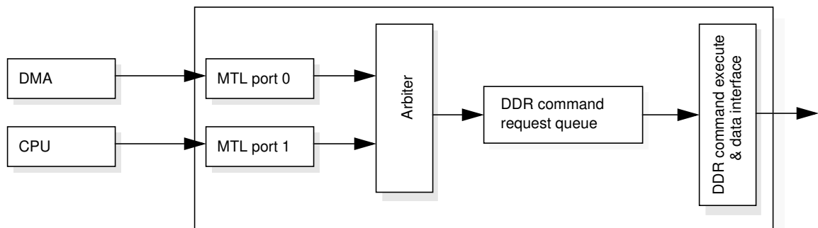
Figure 1: The two MTL Ports of the DDR SDRAM Controller
