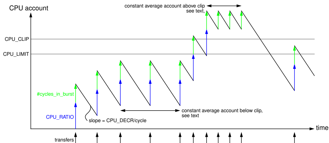
Figure 3: CPU account
