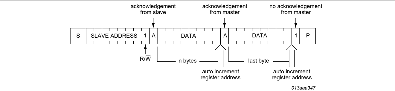
Figure 19. Master reads slave immediately after first byte (READ mode)
