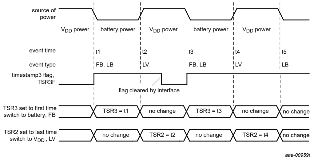
Figure 16. Example battery switch-over timestamp
