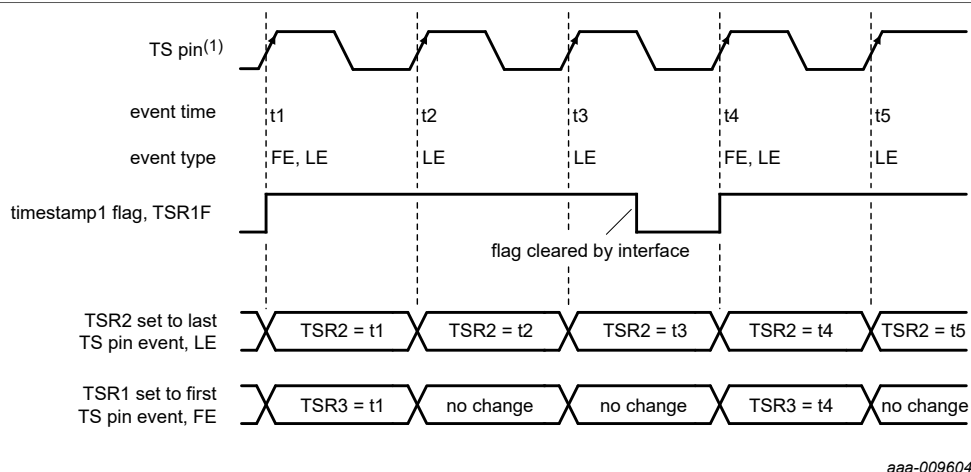
Figure 17. Example TS pin driven timestamp
