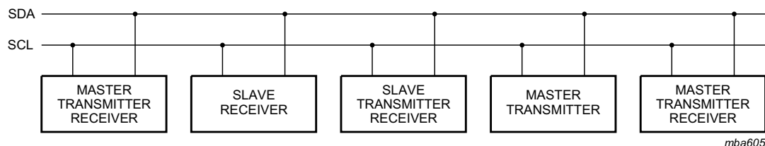
Fig 30. System configuration
