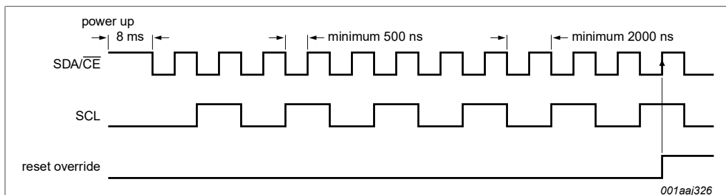
Figure 14. Power-On Reset Override (PORO) sequence, valid for both I 2 C-bus and SPI-bus
