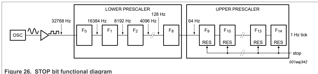
Figure 26. STOP bit functional diagram
