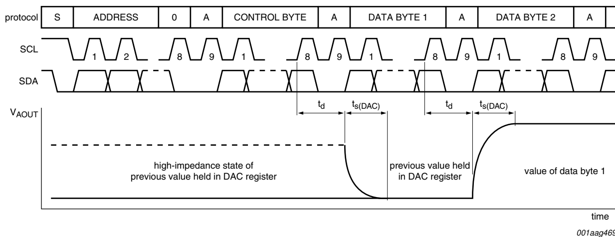
Fig 9. D/A conversion sequence
