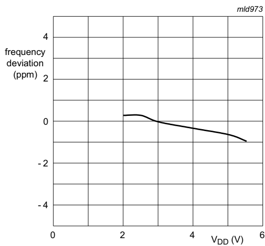
Fig 25. Frequency deviation as a function of V DD
