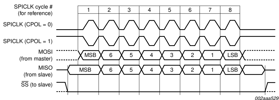
Fig 18. SPI transfer format with CPHA = 0
