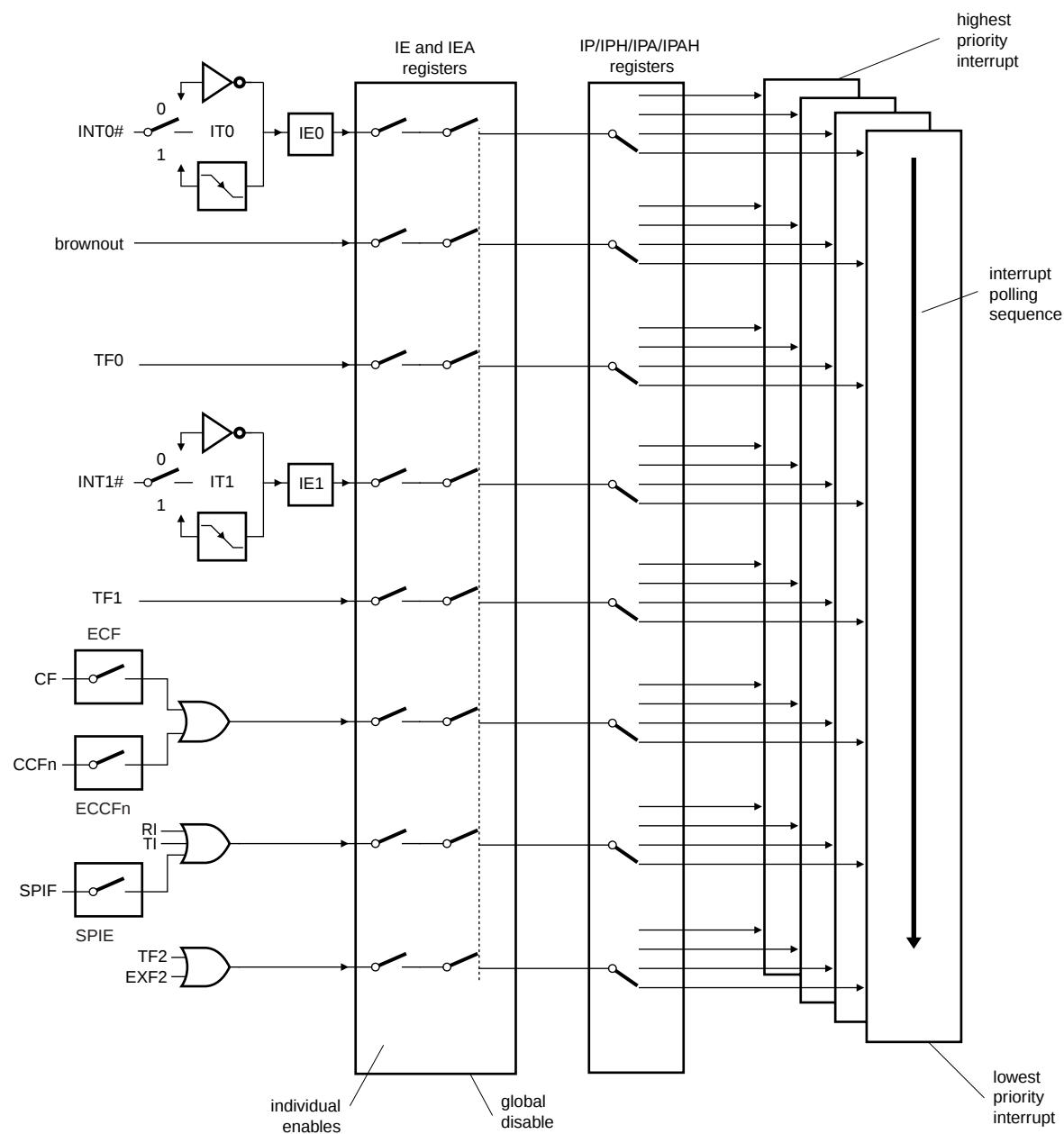
Fig 26. Interrupt structure
