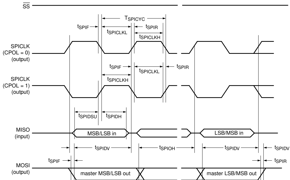
Fig 20. SPI master timing (CPHA = 1)
