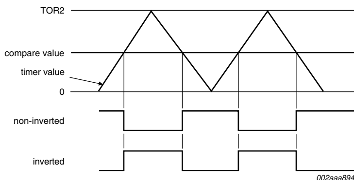
Fig 11. Symmetrical PWM
