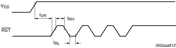
Fig 29. ISP entry timing
