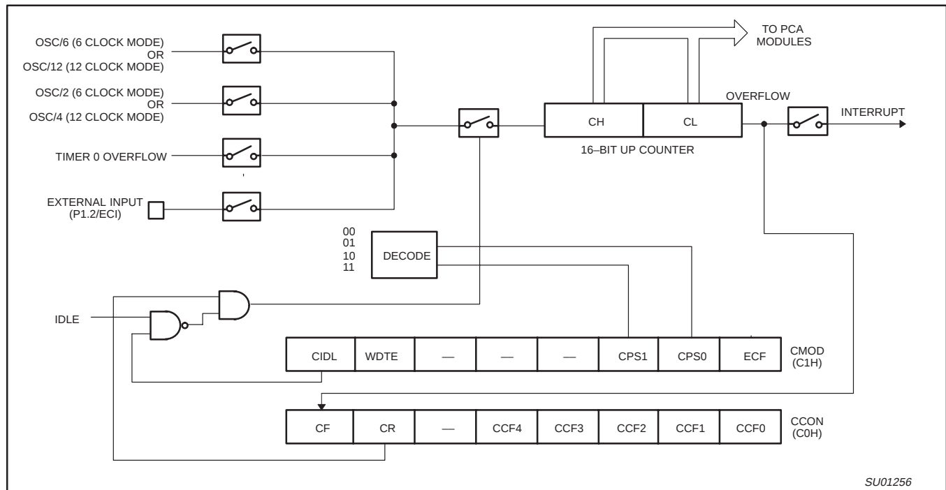
Figure 41. PCA Timer/Counter
