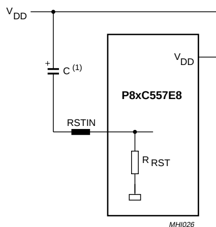
Fig.21 Power-on-reset.
