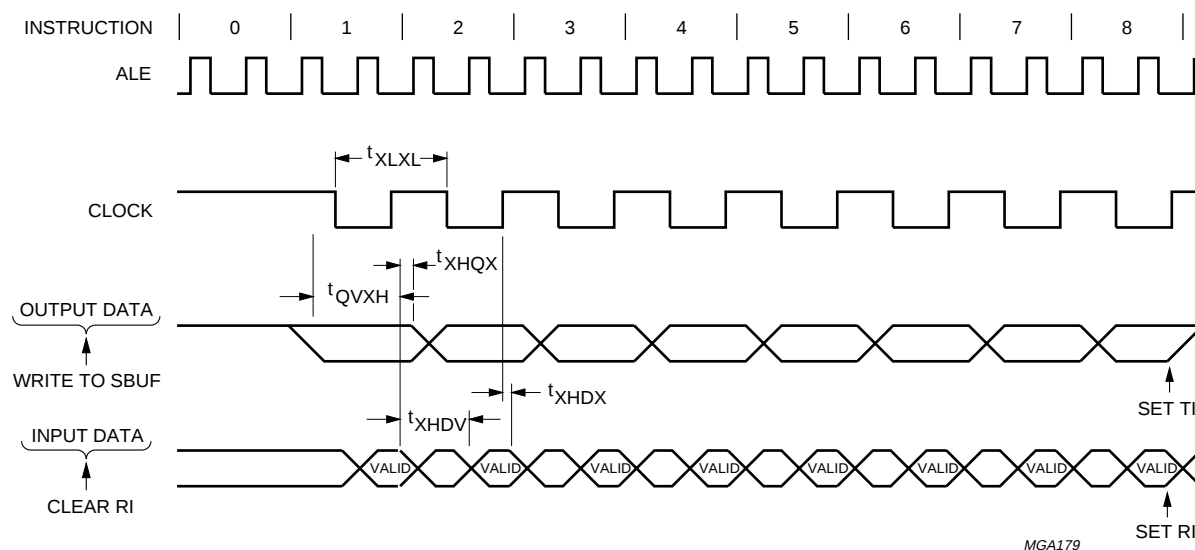
Fig.30 UART waveforms in Shift Register Mode.
