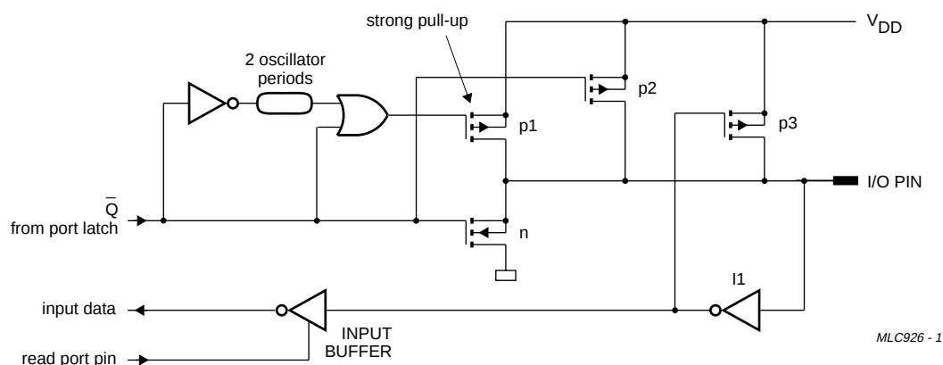
Fig.8 I/O buffers in the P8xC557E8 (Port 1 to Port 4).
