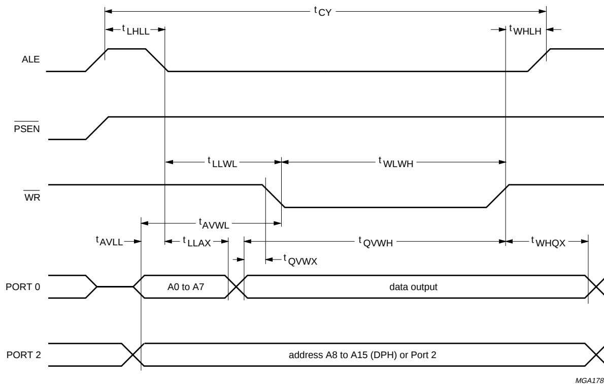
Fig.29 Write to external Data Memory.
