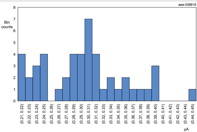
Figure 96. Cout INL
