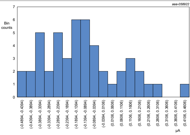
Figure 102. Count user calibrated offset error
