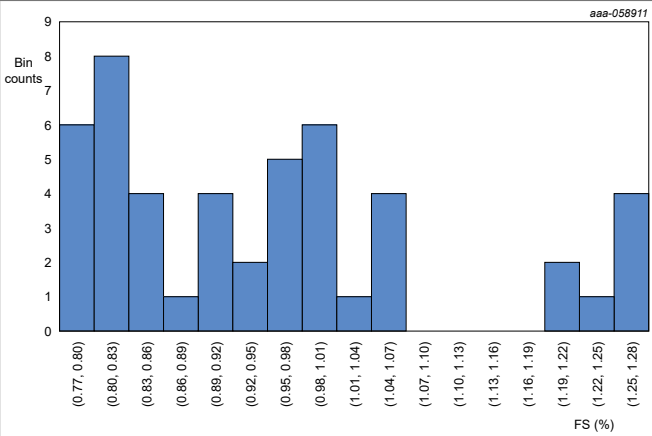
Figure 91. Vout uncalibrated gain error
