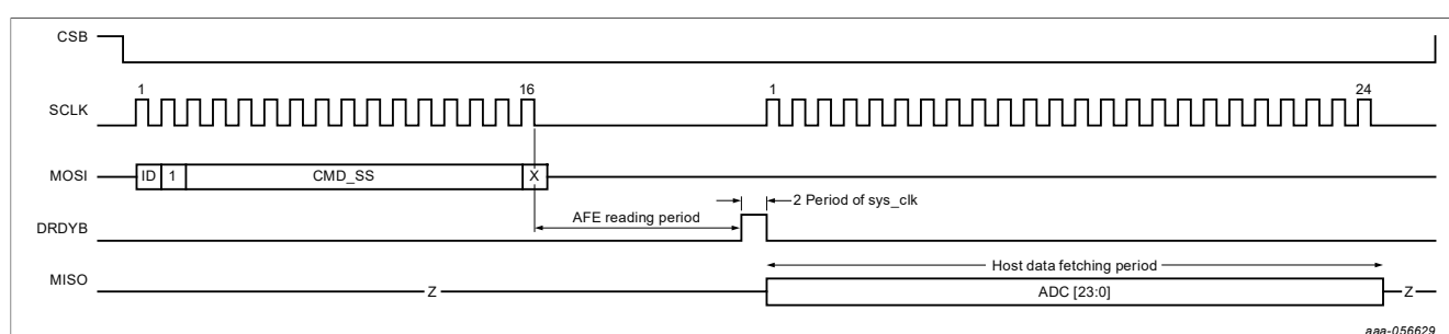
Figure 22. Single-channel single-reading timing diagram with CSB stays low after CMD_SS
