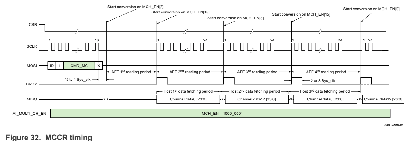
Figure 32. MCCR timing
