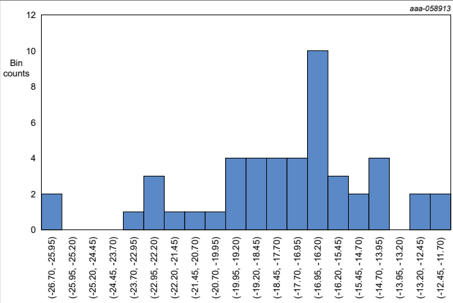
Figure 93. Vout uncalibrated offset error
