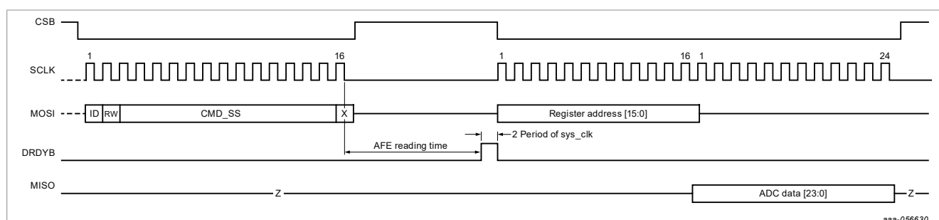
Figure 23. Single-channel single-reading timing diagram with CSB asserts high after CMD_SS
