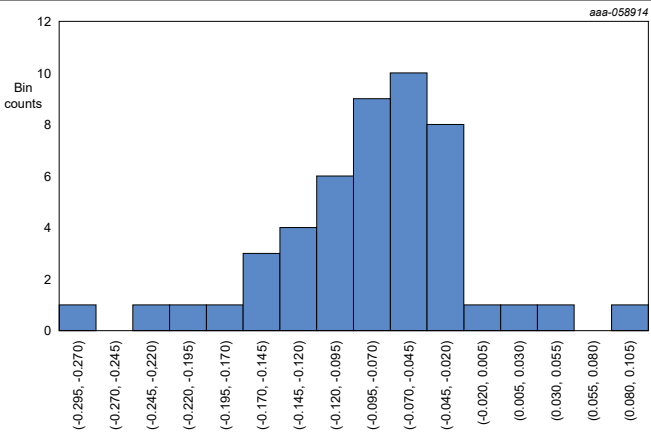
Figure 92. Vout user calibrated gain error
