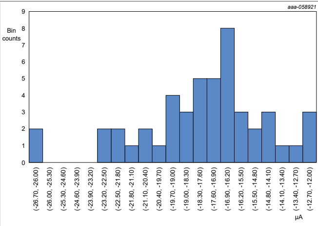
Figure 101. Count uncalibrated offset error
