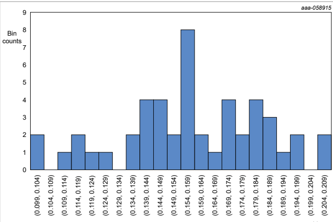
Figure 95. Vout INL
