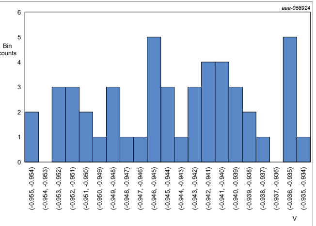
Figure 104. Vout footroom
