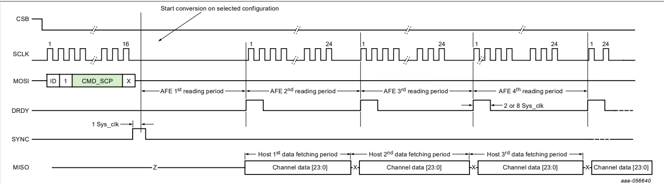
Figure 33. CMD_SC with SYNC trigger timing diagram and CSB low
