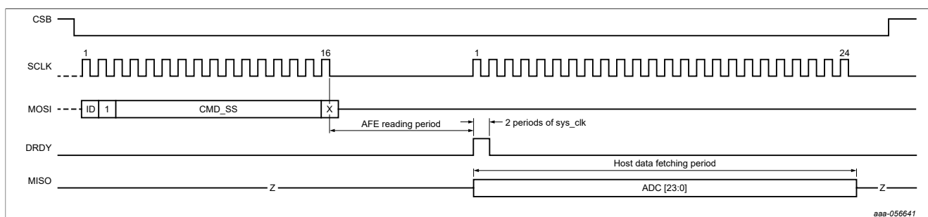
Figure 34. CMD_SS command timing with CSB low
