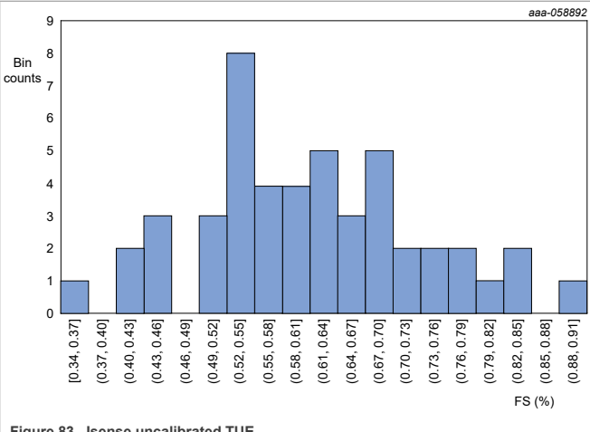
Figure 83. Isense uncalibrated TUE
