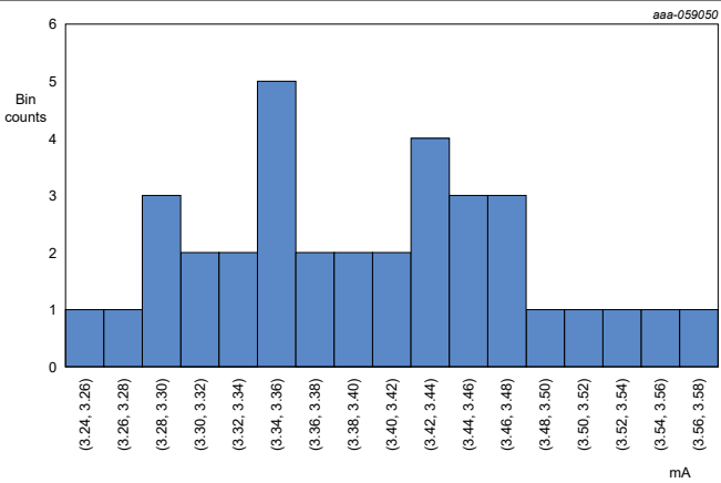
Figure 118. I_HVSS at HVSS = -15 V
