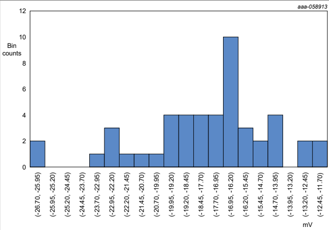
Figure 93. Vout uncalibrated offset error
