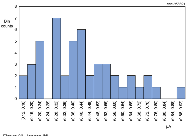
Figure 82. Isense INL
