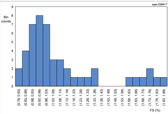
Figure 97. Cout uncalibrated TUE
