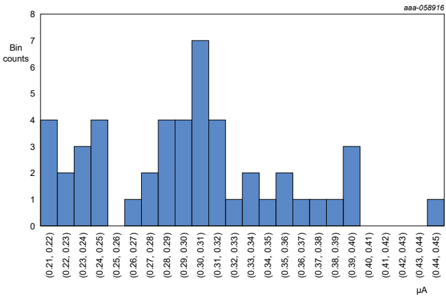
Figure 96. Cout INL
