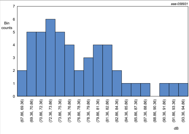
Figure 111. CMRR DC, gain = 1 V/V
