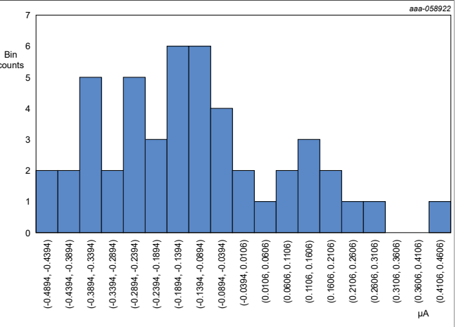
Figure 102. Cout user calibrated offset error
