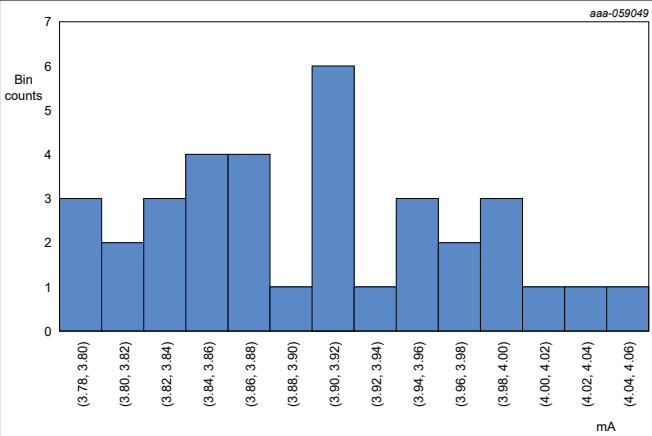
Figure 117. I_HVDD at HVDD = 15 V
