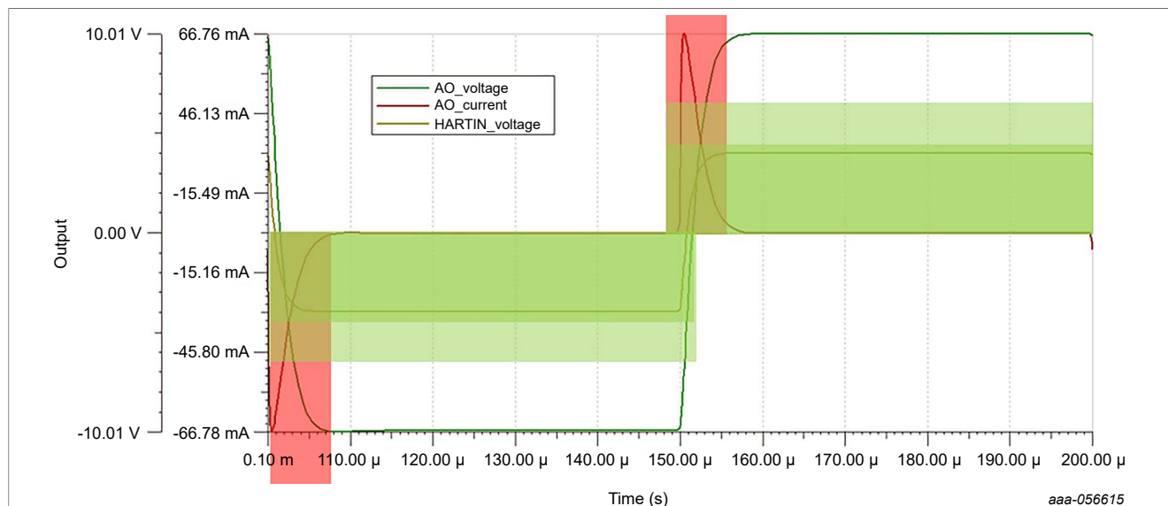
Figure 7. Current output profile in Vout mode with small CL < 10 \text{ nF}
