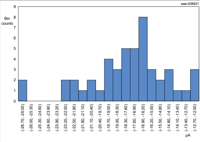
Figure 101. Cout uncalibrated offset error
