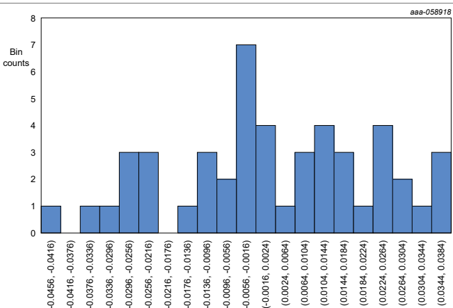
Figure 98. Cout user calibrated TUE
