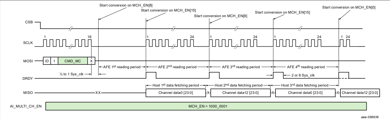
Figure 32. MCCR timing
