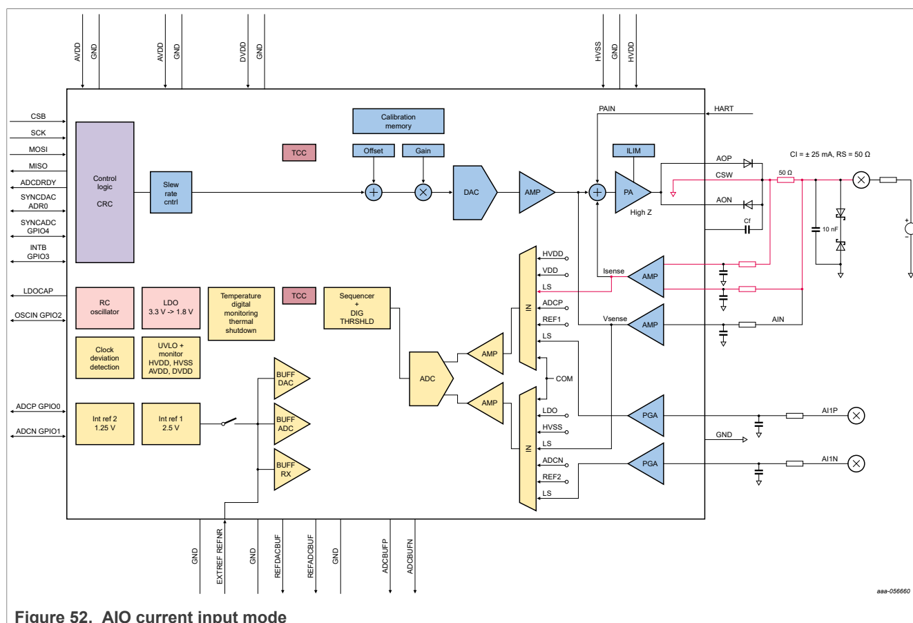
Figure 52. AIO current input mode
