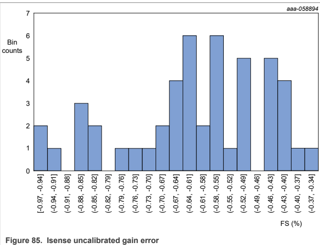
Figure 85. Isense uncalibrated gain error
