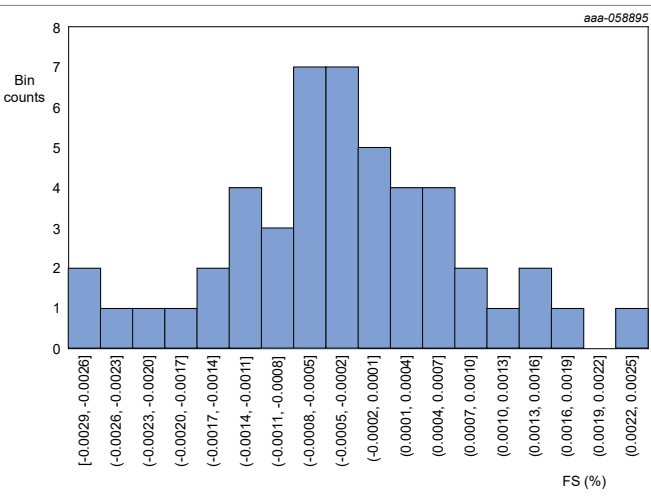
Figure 86. Isense user calibrated gain error
