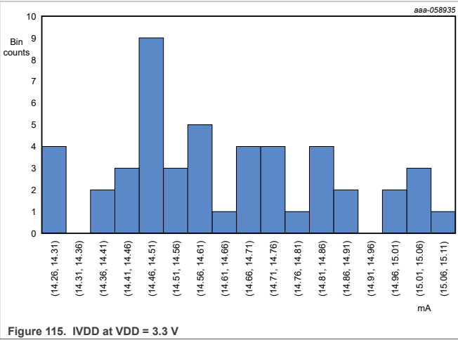
Figure 115. IVDD at VDD = 3.3 V
