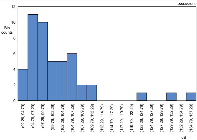
Figure 112. CMRR DC, gain = 16 V/V
