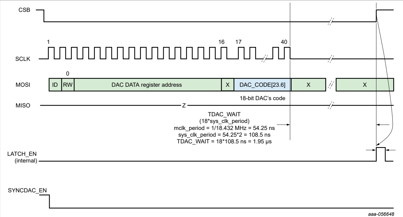
Figure 42. DAC AO_data write timing with CSB
