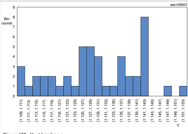
Figure 103. Vout headroom
