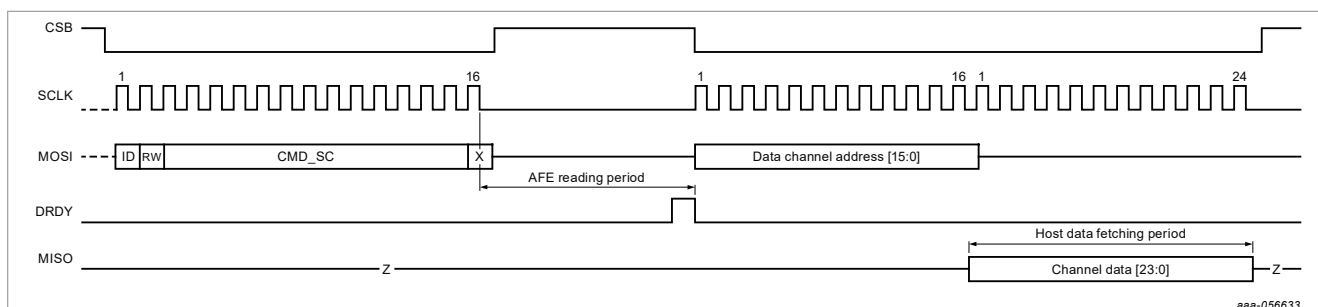
Figure 26. Single-channel continuous-reading timing diagram CSB high
