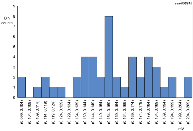
Figure 95. Vout INL
