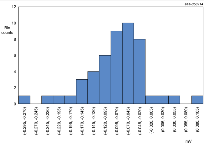
Figure 94. Vout user calibrated offset error
