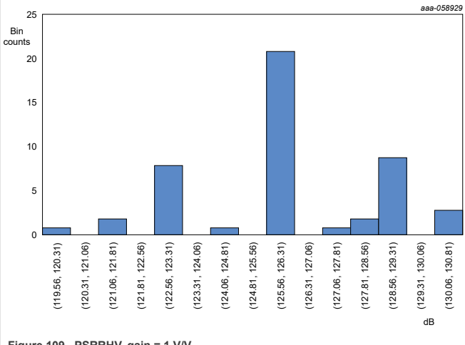
Figure 109. PSRRHV, gain = 1 V/V
