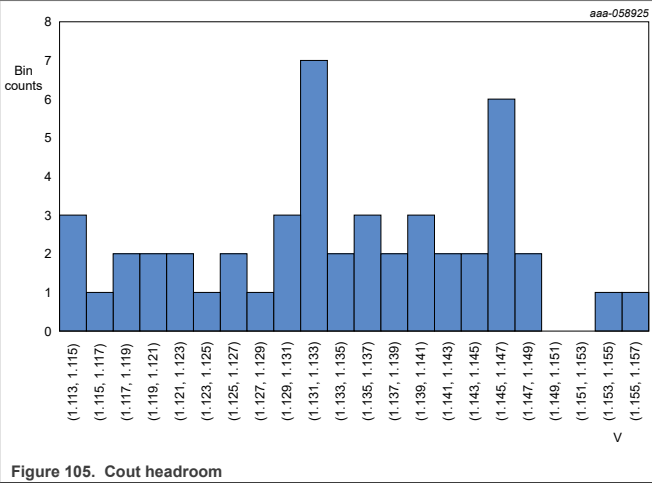
Figure 105. Cout headroom
