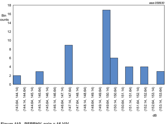
Figure 110. PSRRHV, gain = 16 V/V
