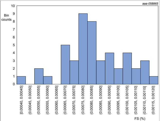
Figure 56. AI1P - VCM user calibrated TUE, PGA = 1V/V
