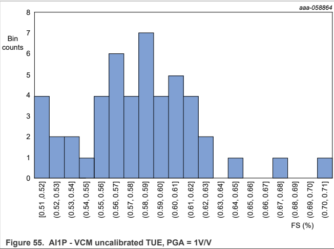
Figure 55. AI1P - VCM uncalibrated TUE, PGA = 1V/V
