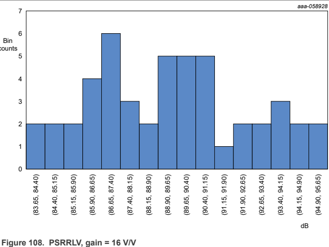
Figure 108. PSRRRLV, gain = 16 V/V
