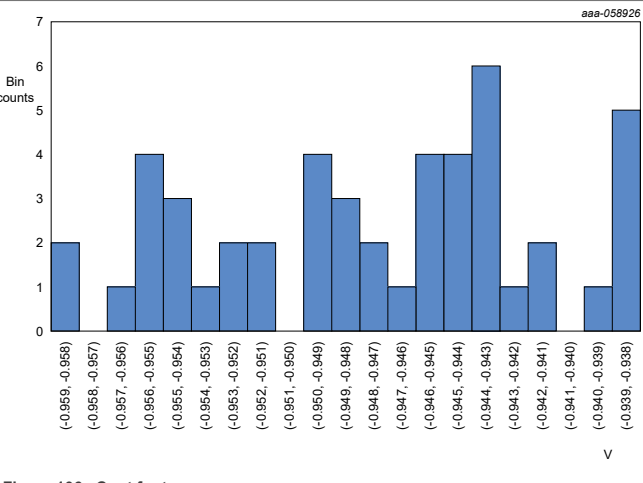
Figure 106. Cout footroom
