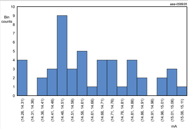
Figure 115. IVDD at VDD = 3.3 V
