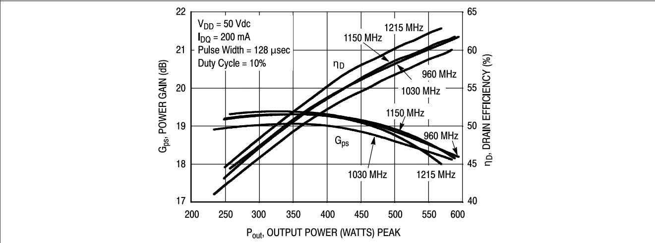
Figure 16. Power Gain and Drain Efficiency versus Output Power
