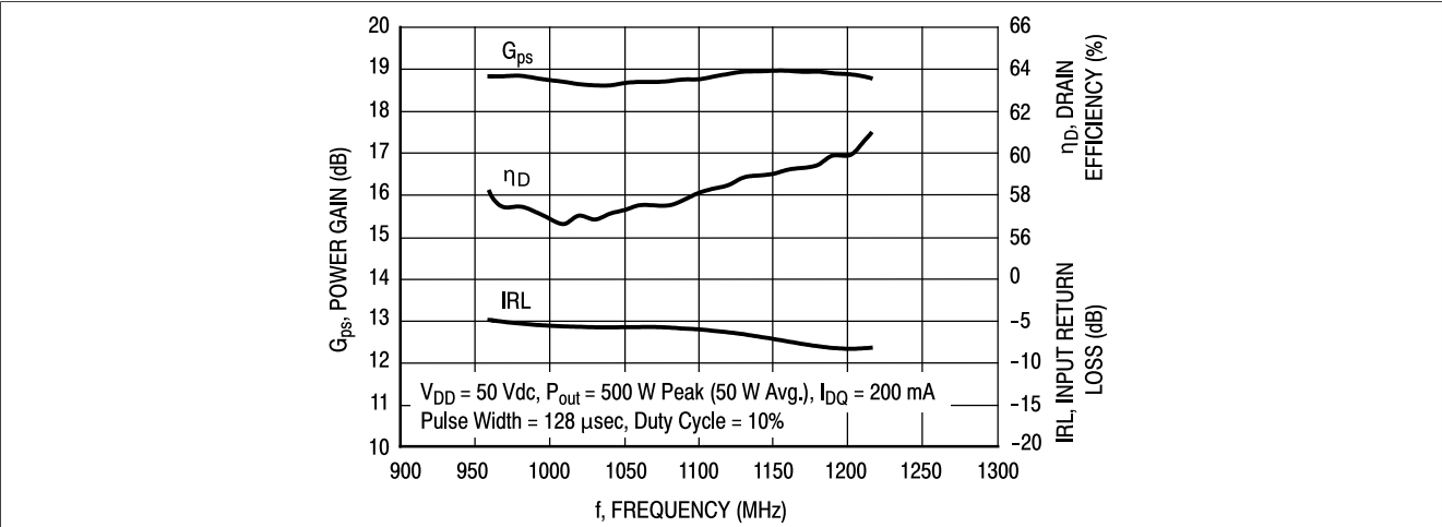
Figure 15. Power Gain, Drain Efficiency and IRL versus Frequency
