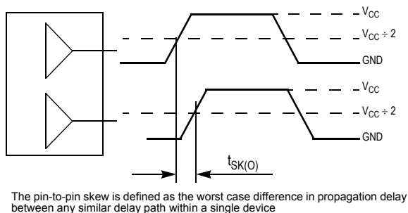
Figure 12. Output-to-Output Skew t_{SK(O)}
