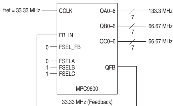
Figure 4. Configuration for 133.3/66.67 MHz clocks
