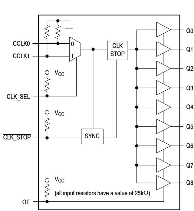
Figure 1. Logic Diagram
