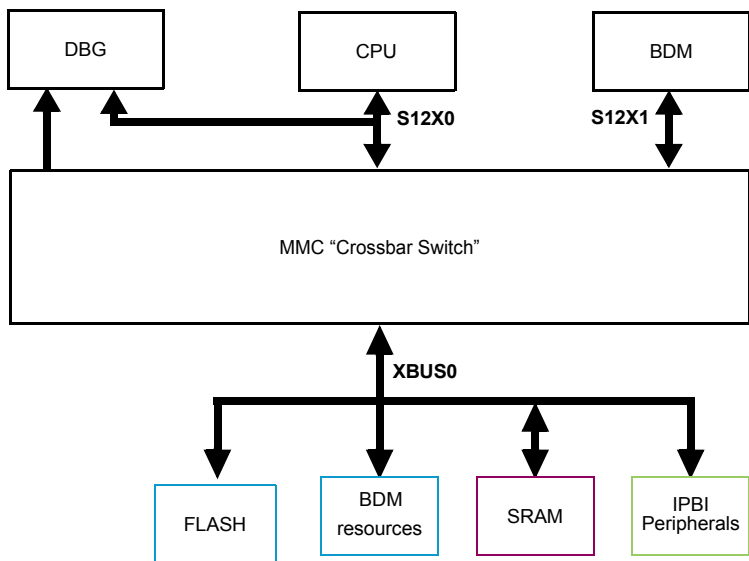
Figure 56. S12S Platform
