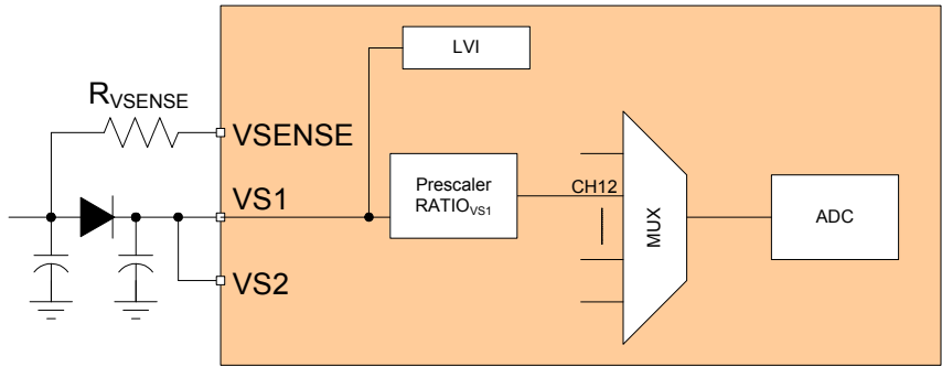
Figure 43. VS1Sense Module
