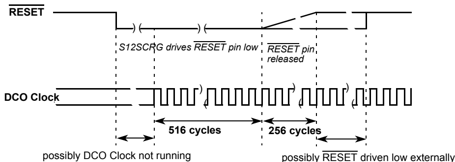
Figure 75. \overline{\text{RESET}} Timing
