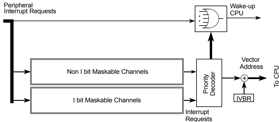
Figure 57. 9S12I32PIMV1 Block Diagram
