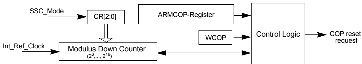
Figure 80. Block Diagram
