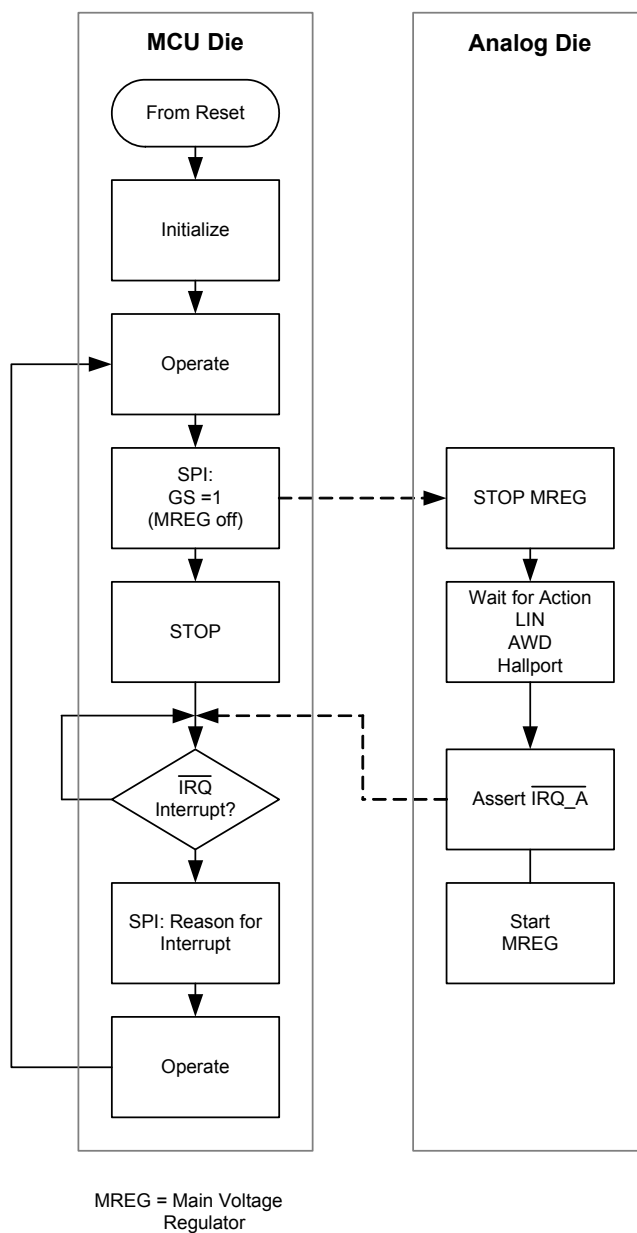
Figure 8. STOP Mode/Wake-up Procedure
