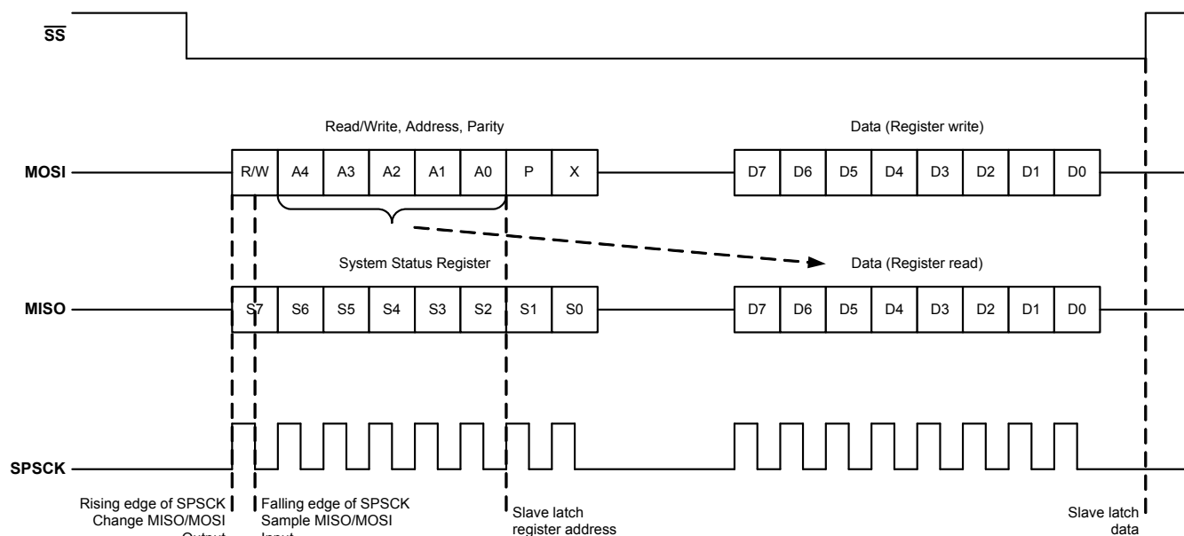
Figure 9. SPI Protocol
