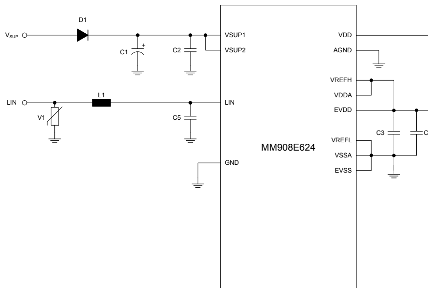
Figure 20. EMC/EMI Recommendations
