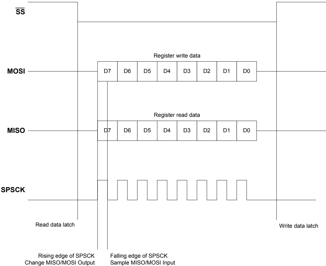
Figure 17. SPI Protocol
