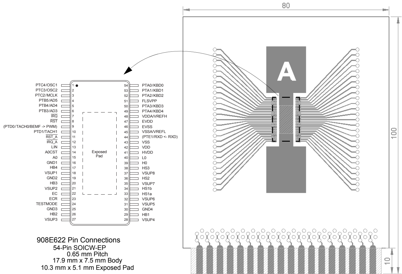
Figure 37. Thermal Test Board
