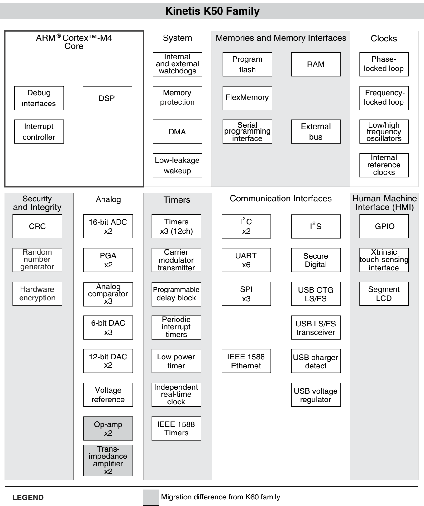
Figure 2. K50 Block Diagram
