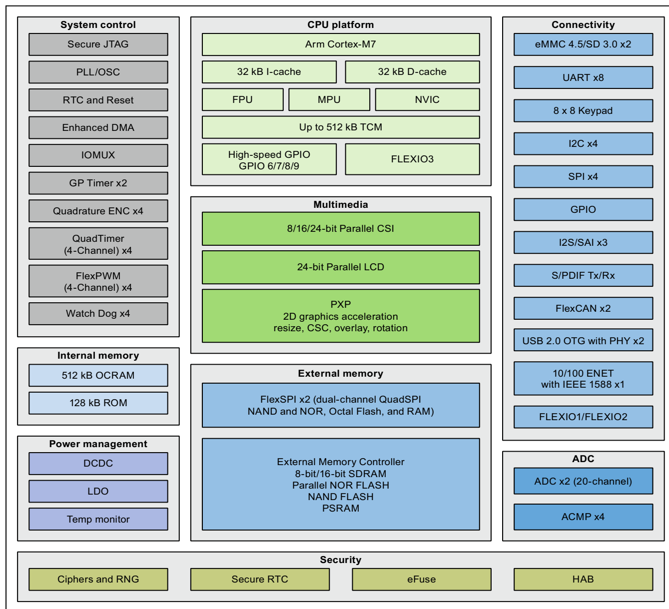
Figure 2. i.MX RT1060 system block diagram
