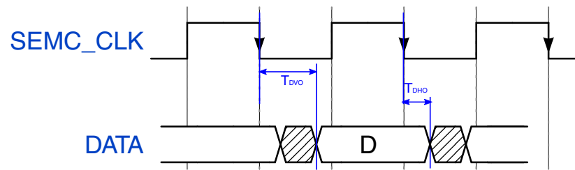
Figure 16. SEMC output timing in SYNC mode
