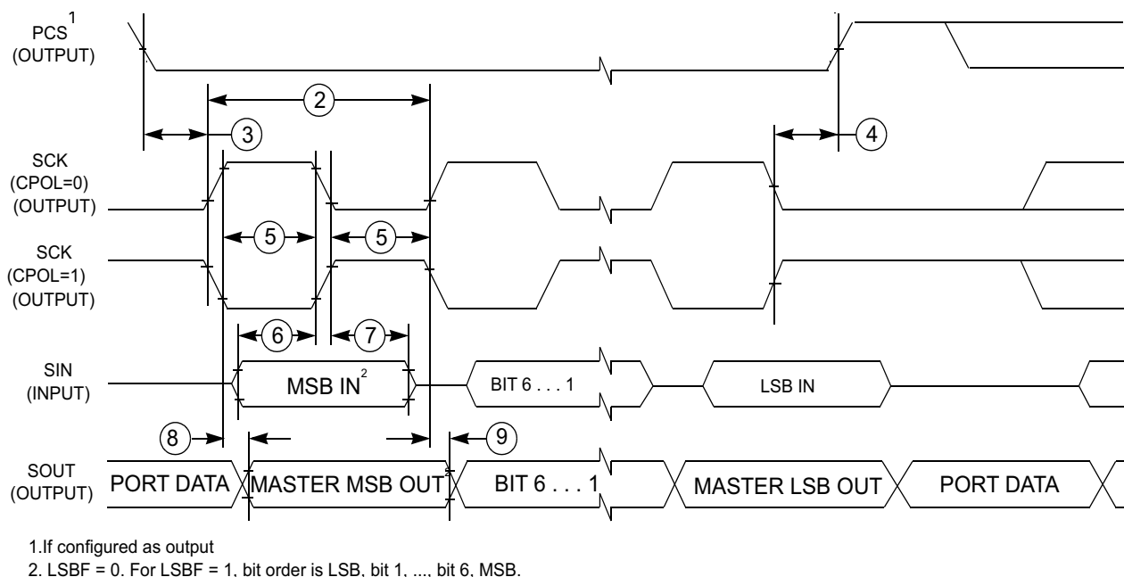
Figure 40. LPSPI Master mode timing (CPHA = 1)
