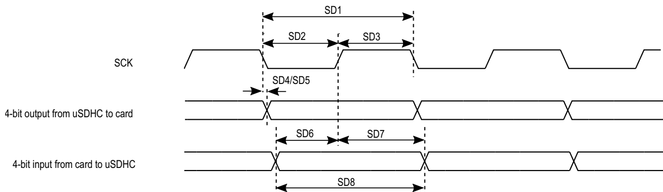
Figure 45. SDR50/SDR104 timing
