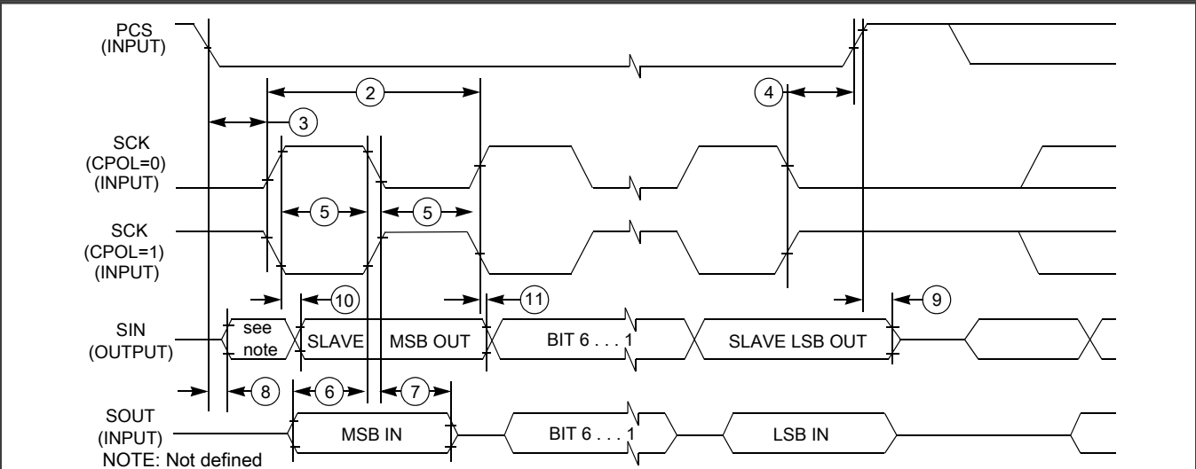
Figure 42. LPSPi Slave mode timing (CPHA = 1)
