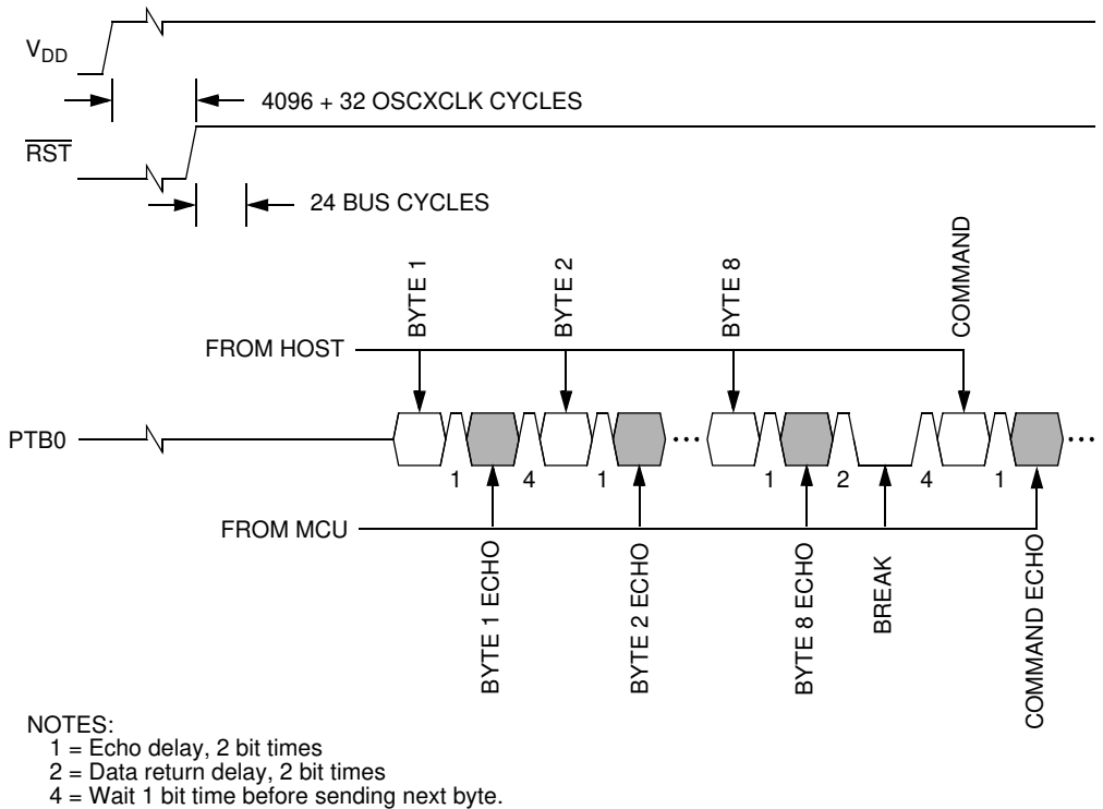
Figure 9-7. Monitor Mode Entry Timing
