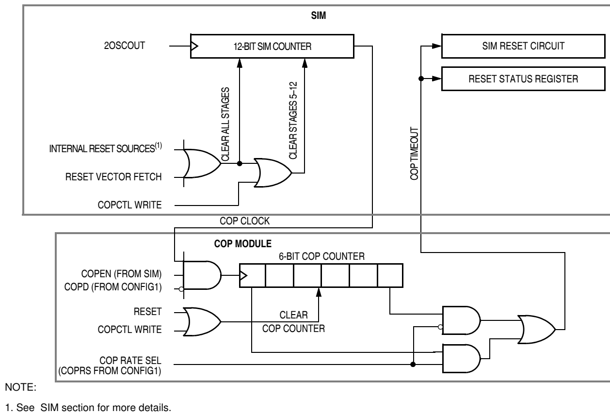
Figure 15-1. COP Block Diagram
