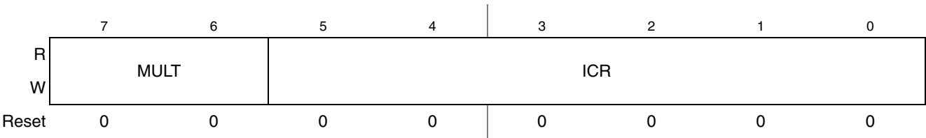
Figure 13-4. IIC Frequency Divider Register (IIC1F)
