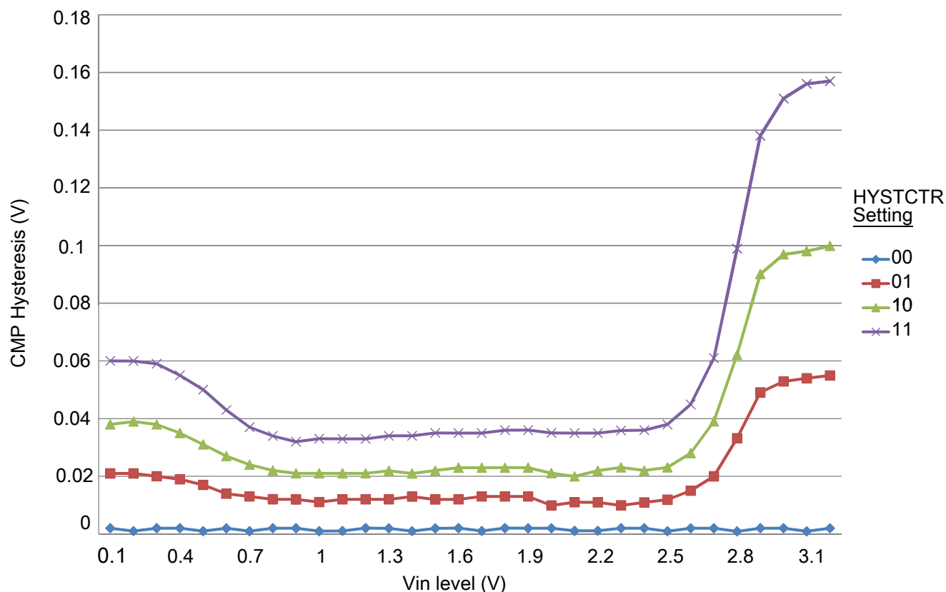
Figure 12. Typical hysteresis vs. Vin level ( V_{DD} = 3.3\text{ V} , P\text{MODE} = 1 )
