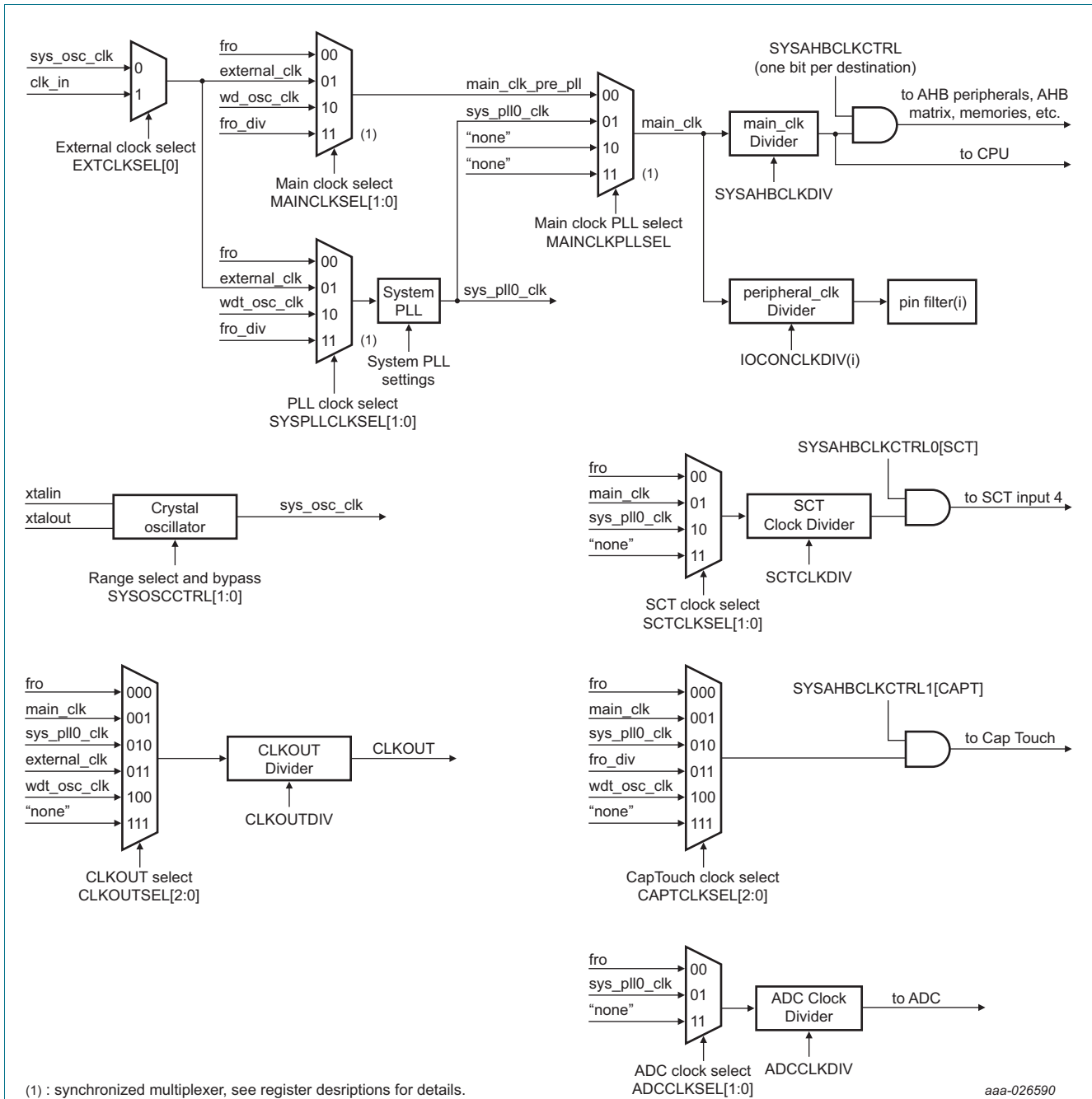
Fig 11. LPC84x clock generation
