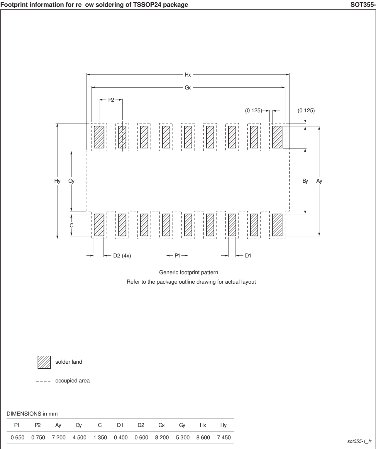
Fig 40. Reflow soldering of the TSSOP24 package
