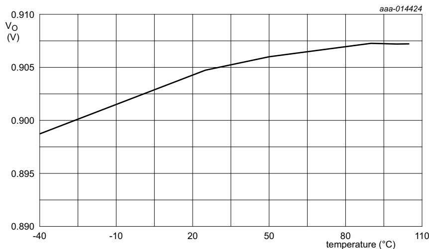
Fig 32. Typical internal voltage reference output voltage
