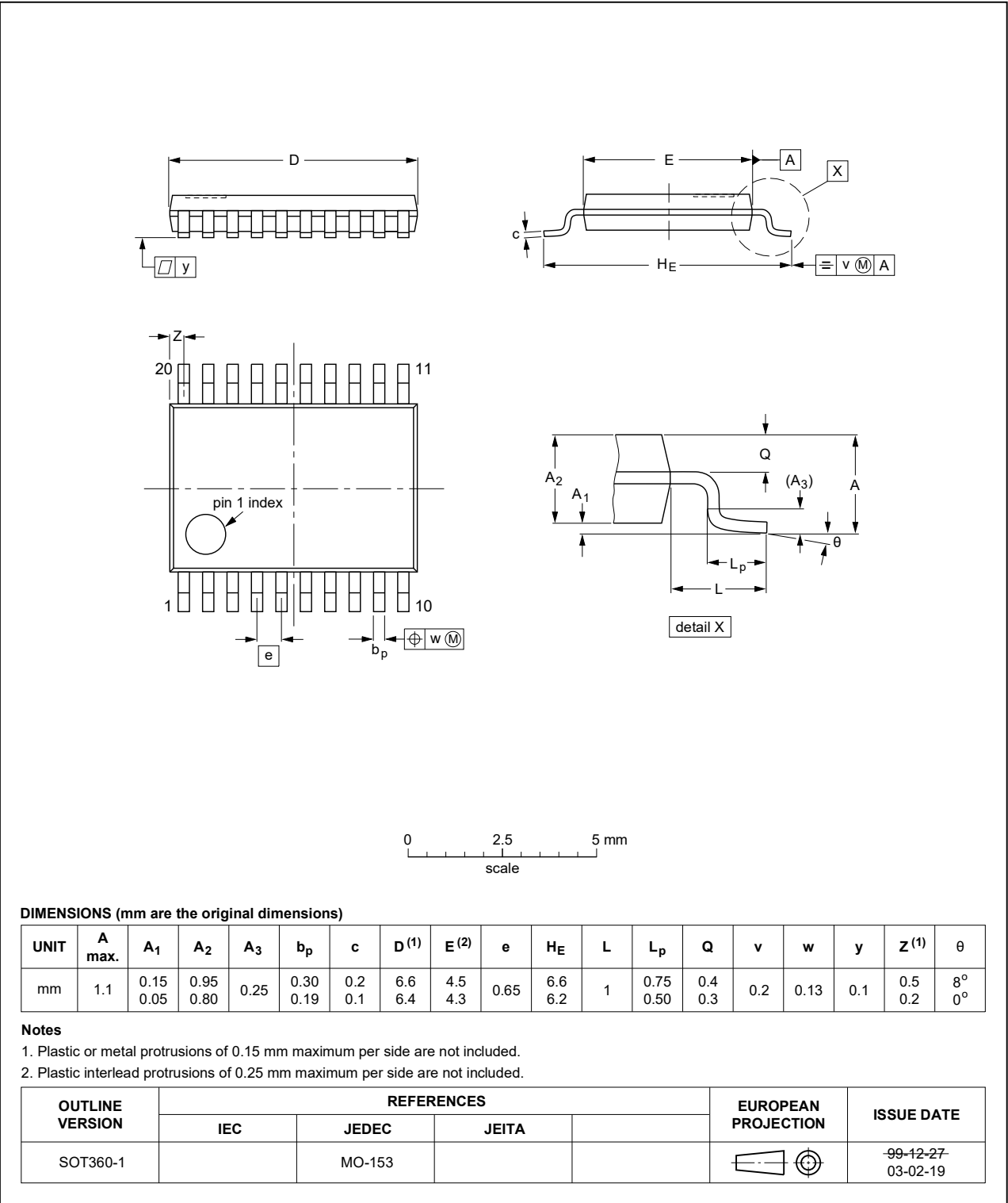
Figure 35. Package outline SOT360-1 (TSSOP20)
