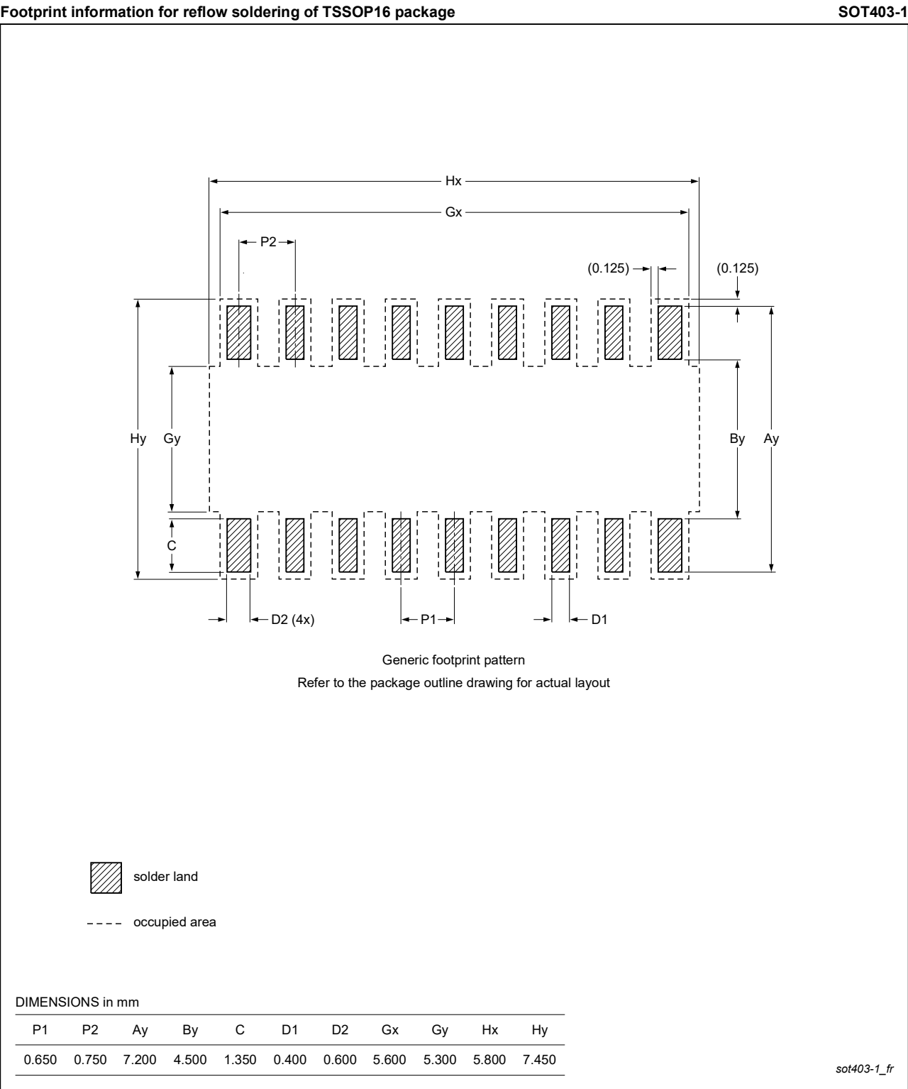
Figure 40. Reflow soldering of the TSSOP16 package
