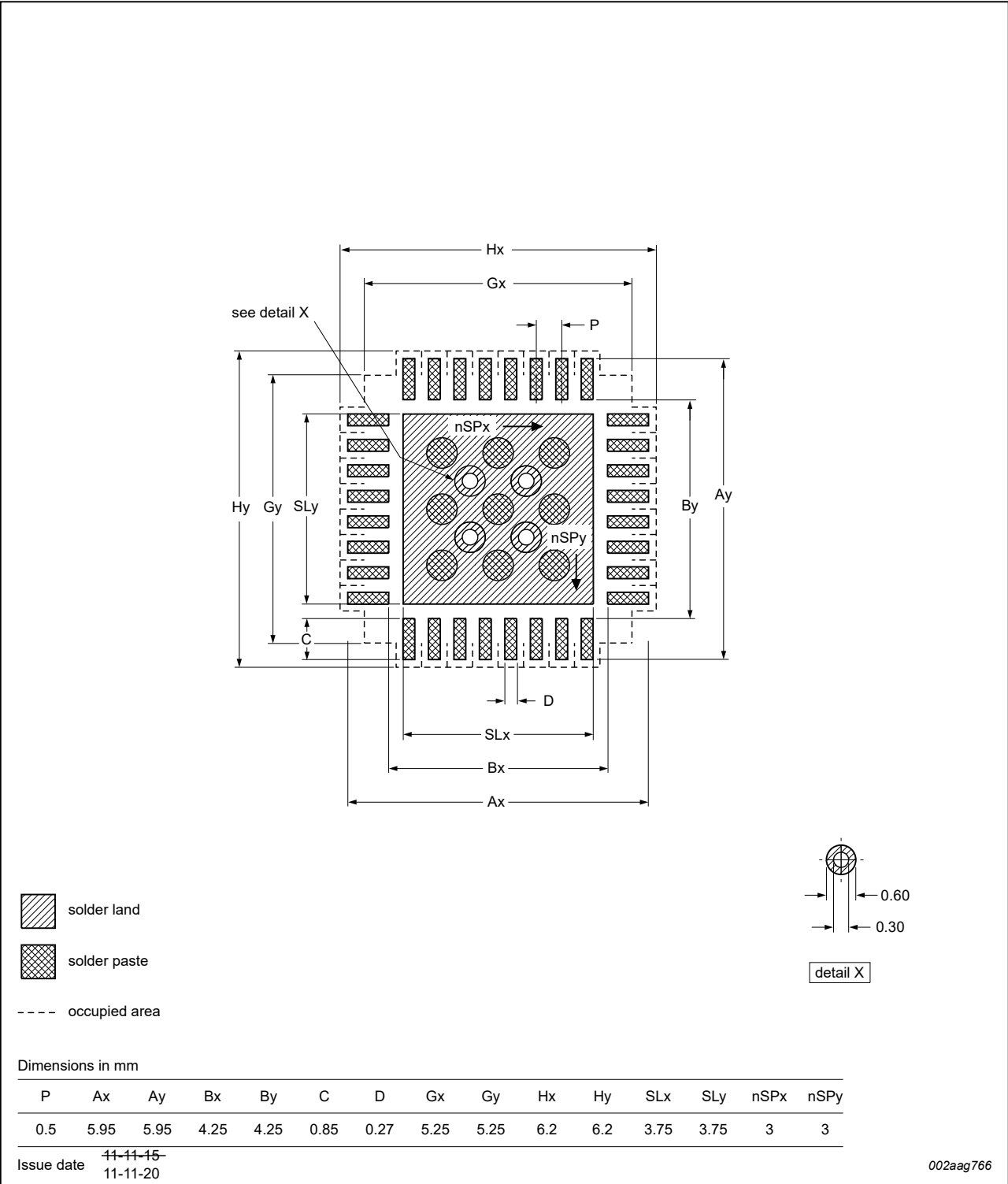
Figure 41. Reflow soldering for the HVQFN33 (5x5) package
