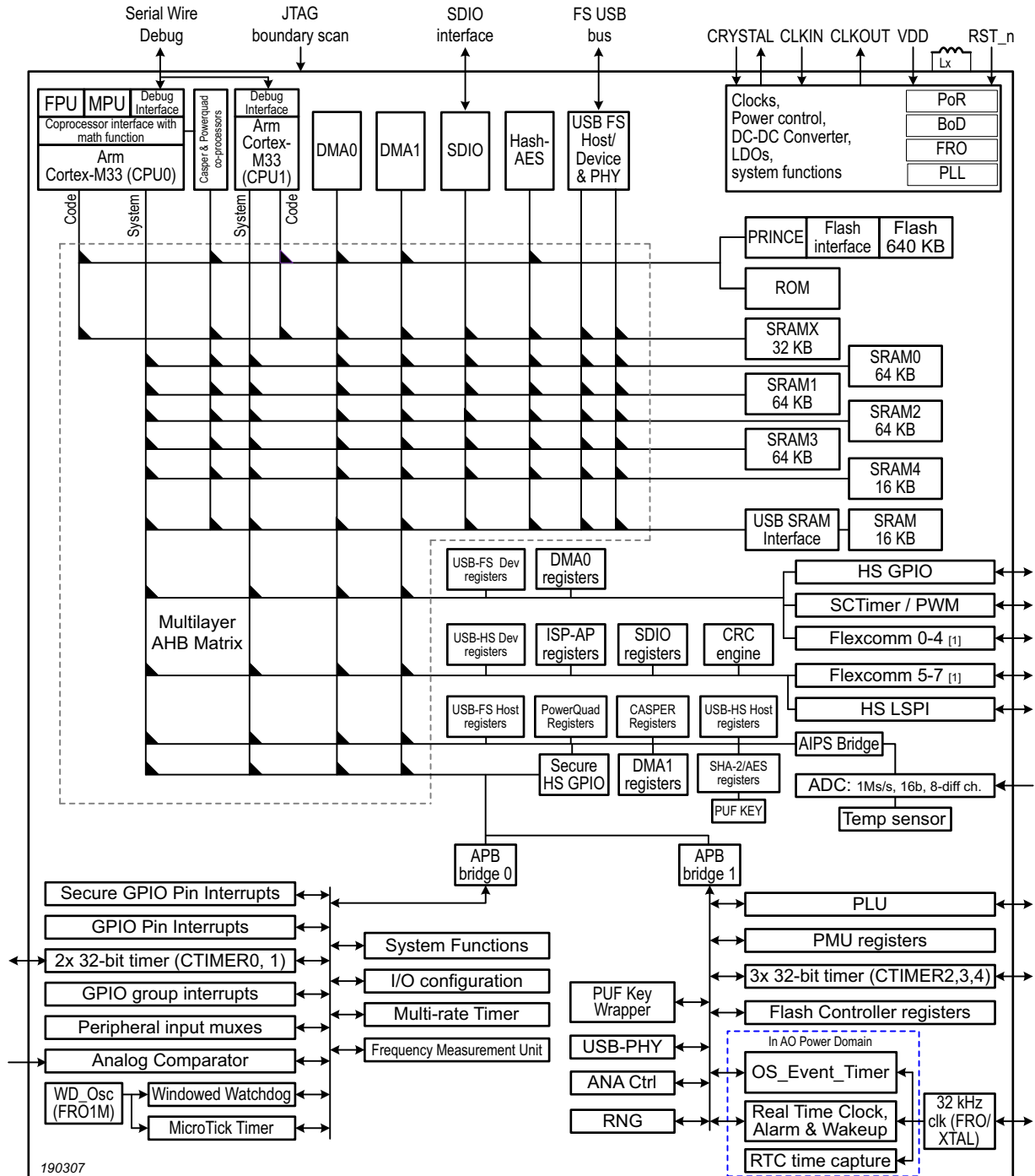
Fig 4. LPC55S6x Block diagram
