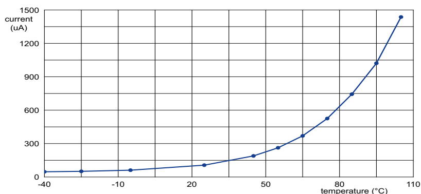
Fig 9. Deep-sleep mode: Typical supply current I_{DD} versus temperature for different supply voltages VBAT_DCDC
