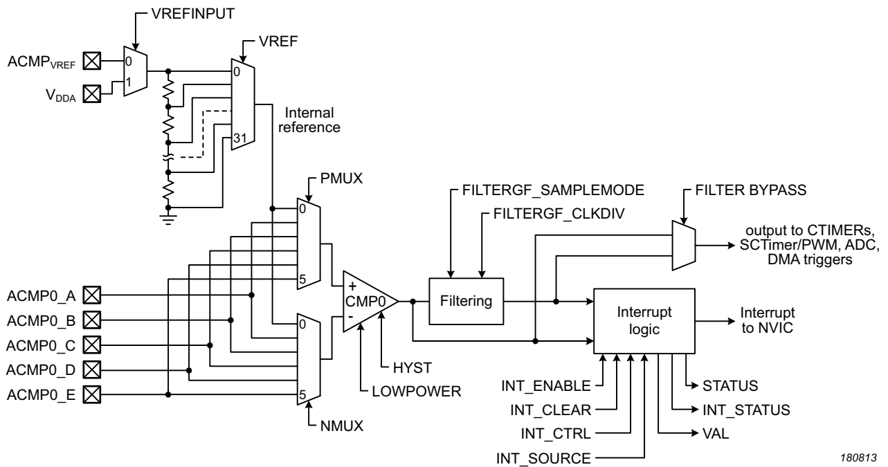
Fig 8. Comparator block diagram
