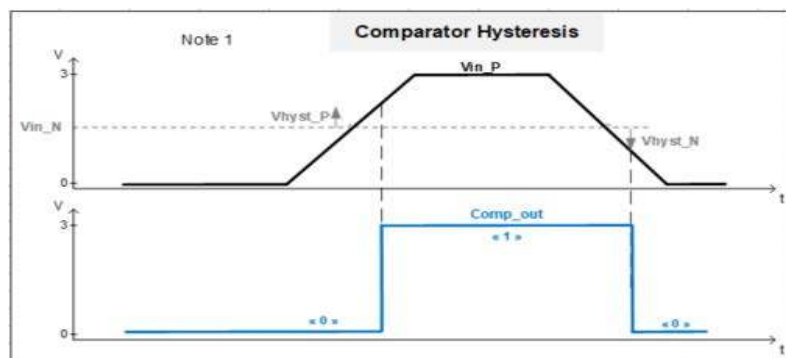
Fig 20. Comparator Hysteresis
