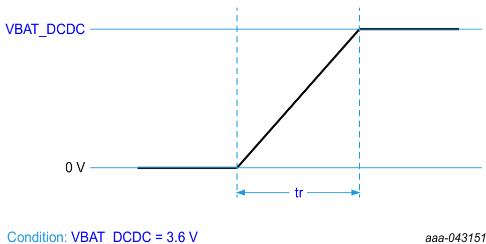
Fig 10. Power-up ramp
