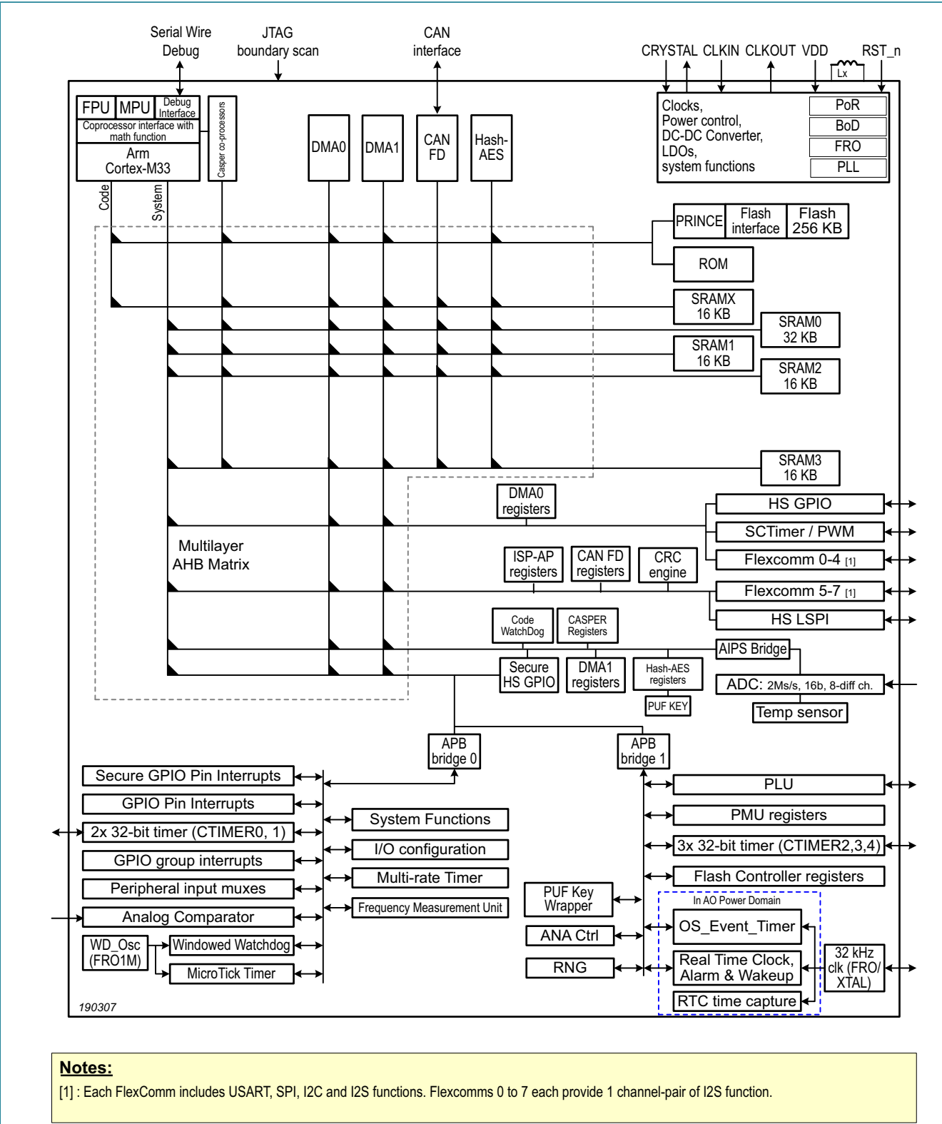
Fig 2. LPC55S0x/LPC550x Block diagram
