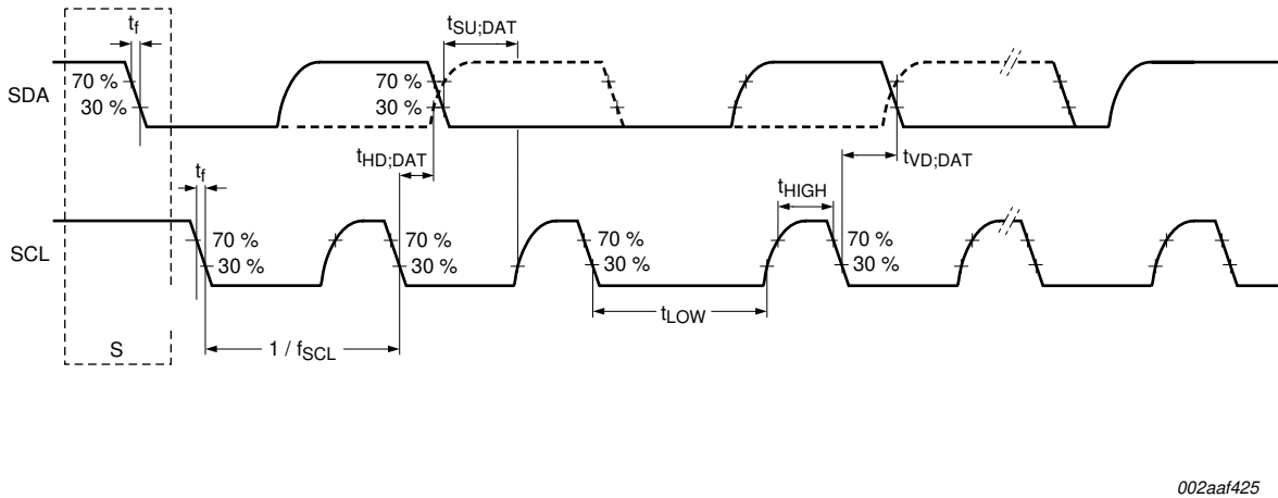
Fig 28. I 2 C-bus pins clock timing
