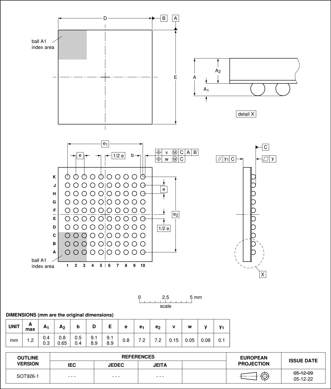
Fig 53. TFBGA100 package
