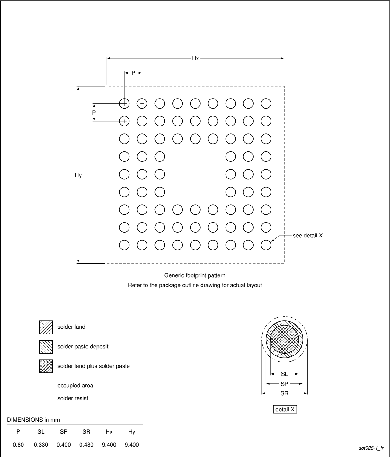
Fig 58. Reflow soldering of the TFBGA100 package
