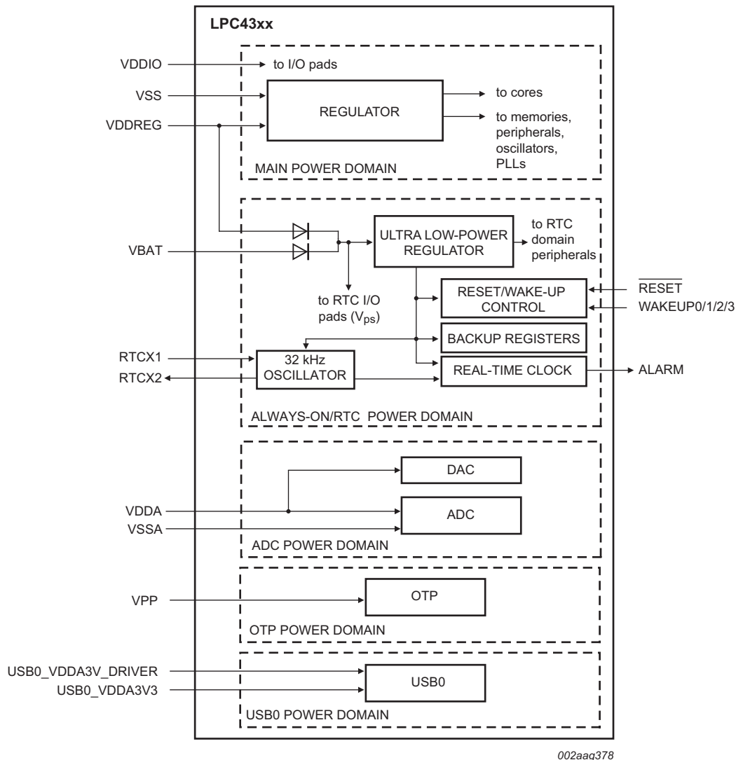
Fig 9. Power domains
